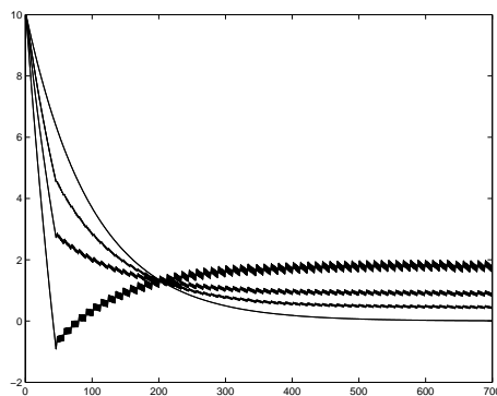
FIGURE 3. State trajectory for the system of Fig. 2. Chattering around the hyperplane \mathcal{H} is due to the discontinuous behavior of \omega that jumps between \bar{\omega} and -\bar{\omega} .
