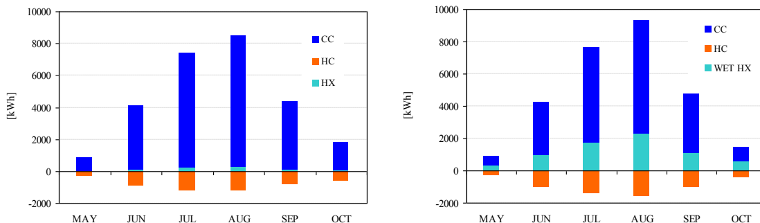
Fig. 7. Energy distribution in the AHU equipped with sensible heat exchanger (left) and wet heat exchanger (right)
