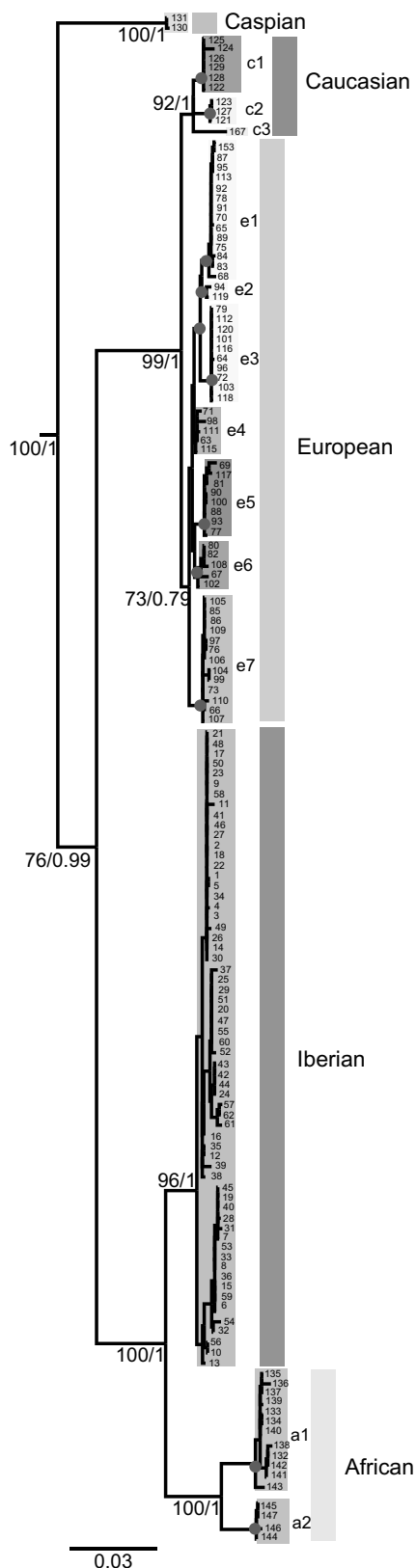
Fig. 2. Phylogenetic relationships of the Bufo bufo species complex in the Western Palearctic, as inferred from the ML analysis of 1988 bp of mtDNA. The support values (bootstrap/pp) are shown next to the nodes of the major splits. The red dots depicted in the shallow splits denote a bootstrap value equal or higher than 80% and simultaneously a posterior probability equal or higher than 0.90. The reference bar is expressed in substitutions per site. Numbers at the tips of the tree refer to specimens listed in Table 1. The outgroups have been removed. (For interpretation of the references to color in this figure legend, the reader is referred to the web version of this article.)
