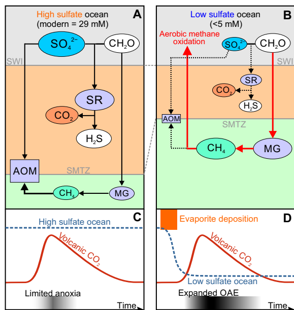
Fig. 4. Conceptual model of the methane-oxygen link under high and low sulfate conditions. (A) The fate of organic carbon in the modern high sulfate ocean: More organic carbon and methane are oxidized by sulfate with negligible benthic methane flux, which limits water column oxygen demand. (B) The effect of enhanced methanogenesis in a low sulfate setting: The proportion of organic carbon available for methane production is increased, sulfate-driven anaerobic AOM oxidation is suppressed, and methane production moves closer to the sediment surface producing a high benthic oxygen demand. Red arrows in (B) indicate acceleration of biogeochemical pathways relative to modern, whereas dotted black arrows indicate retardation. (C and D) The envisaged oxygen depletion responses of the ocean to the same \text{CO}_2 forcing under high and low sulfate conditions. Sulfate is thought to be removed by evaporite deposition. Marine anoxia is exacerbated by the increased oxygen demand as net seafloor methane fluxes increase during warming. MG, methanogenesis. SMTZ, sulfate-methane transition zone.
