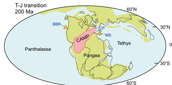
Fig. 1. Simplified paleogeographical map for Triassic–Jurassic transition showing localities for all three studied sections. This figure is modified after the work of Luo et al. (16). T–J, Triassic–Jurassic. Yellow filled triangles indicate the location of studied sections. The paleogeographical location and the extent of CAMP are based on the work of Marzoli et al. (42).
