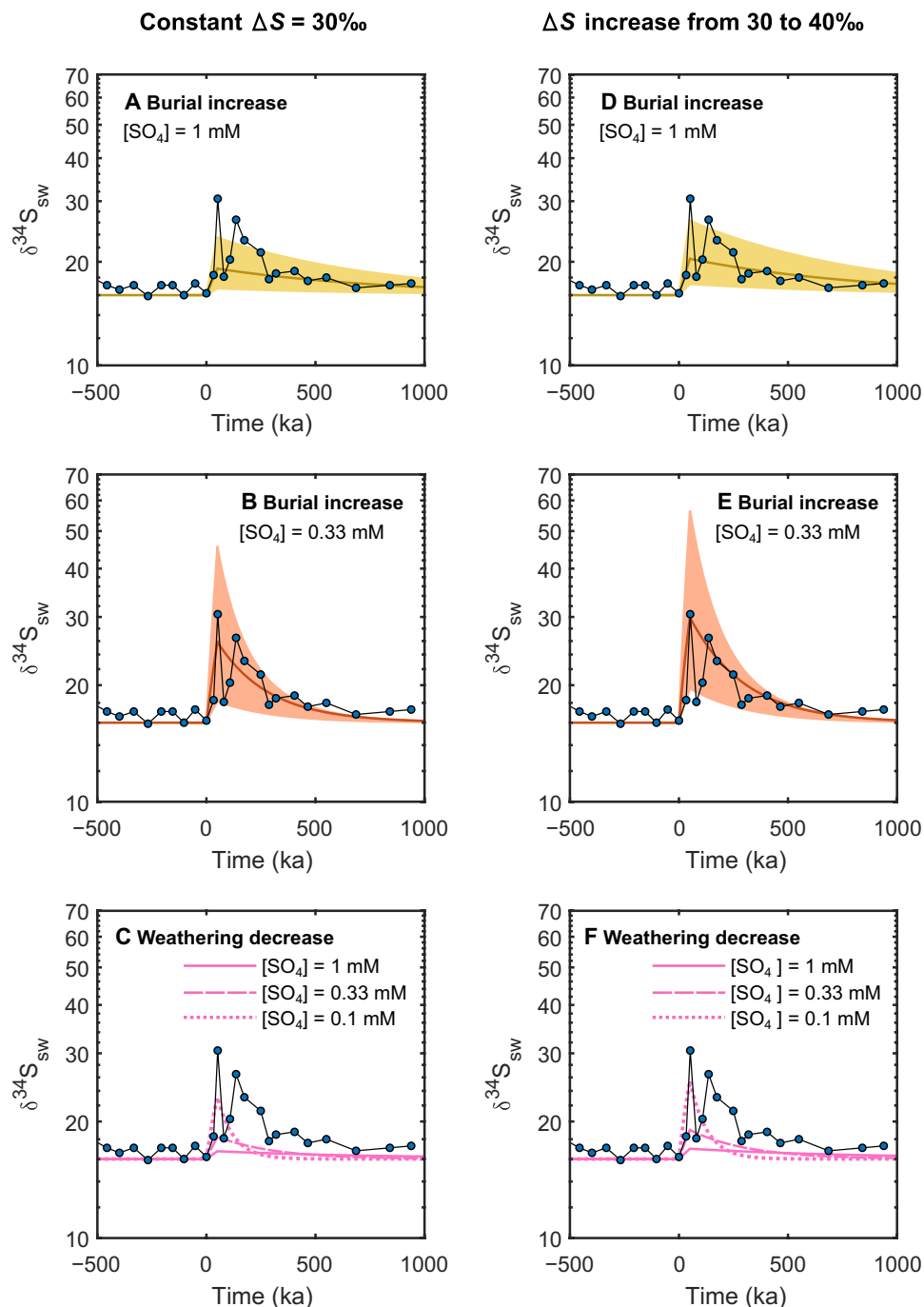
Fig. 3. Sulfur cycle box model outputs. (A and B) Increased in the pyrite burial rate under different values for the starting oceanic sulfate inventory, with tests of 1 mM (A) (yellow) and 0.33 mM (B) (red). For both scenarios, a step increase in pyrite burial is assumed to occur at t = 0 over a period of 50 ka, which represents the ETME. Both models assume the same increase in pyrite burial rates, which ranges from 2- to 10-fold to create the shaded area, with the centerline showing a fivefold increase. The best fit to the data occurs for marine sulfate concentration [\text{SO}_4] = 0.33 \text{ mM} (B). (C) Attempts to fit the \delta^{34}\text{S}_{\text{CAS}} data by instead reducing the pyrite weathering rate to zero over the same 50-ka time frame. Here, regardless of [\text{SO}_4] , the shape of the curve cannot be fit. This is because creating the large excursion this way requires extremely low [\text{SO}_4] , and, in these circumstances, the system is quick to regain isotopic stability. (D to F) Repetition of these experiments with the addition of a change in the enrichment factor \Delta S between oceanic sulfate and sedimentary pyrite and continuation to produce a better fit when [\text{SO}_4] = 0.33 \text{ mM} .
