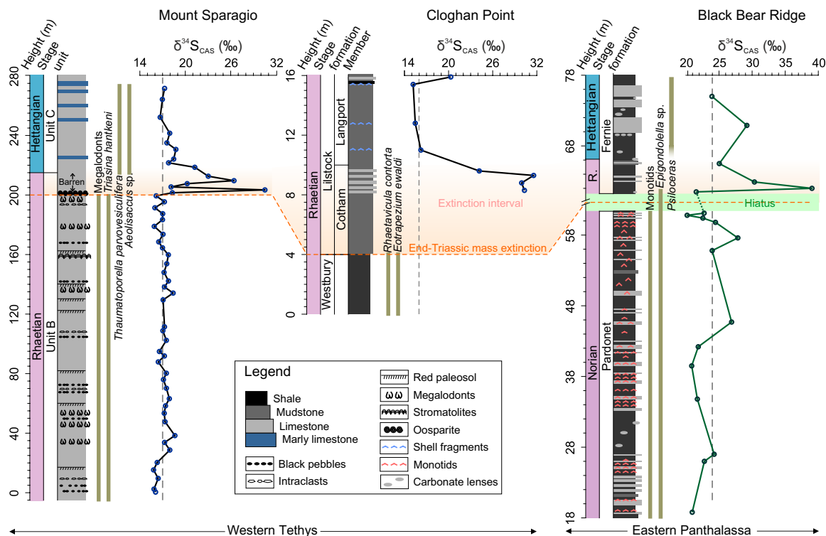
Fig. 2. \delta^{34}\text{S}_{\text{CAS}} profiles from Late Triassic to Early Jurassic for the three studied sites of the Tethys and Panthalassa oceans. R., Rhaetian. The orange shadowed field indicates the extended extinction interval following the major mass extinction horizon. The light green field indicates a hiatus between Norian and Rhaetian at the BBR. Dark green bars represent the fossil occurrence ranges. See the Supplementary Materials for further stratigraphic details. Vertical dash lines indicate pre- or post-excursion average baseline values.
