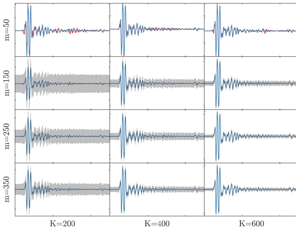
Figure 6: Effect of compressed signal size and dictionary size on confidence intervals of an illustrative ultrasound pulse. This prediction uses a k-means dictionary. m denotes the compressed dimension while K denotes the dictionary size. The original dimension was 1232 data points.
