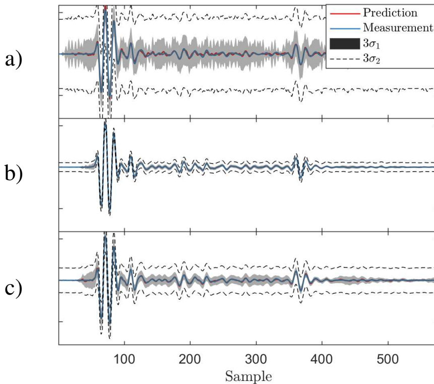
Figure 5: Comparison of predictions on ultrasound data using three different dictionaries: a) model-based tone-burst, b) k-means clustering and c) online matrix factorisation. Two different uncertainty bounds are shown: \sigma_1 shows predictive variance without the noise term, whilst \sigma_2 shows the result of the additive noise term.
