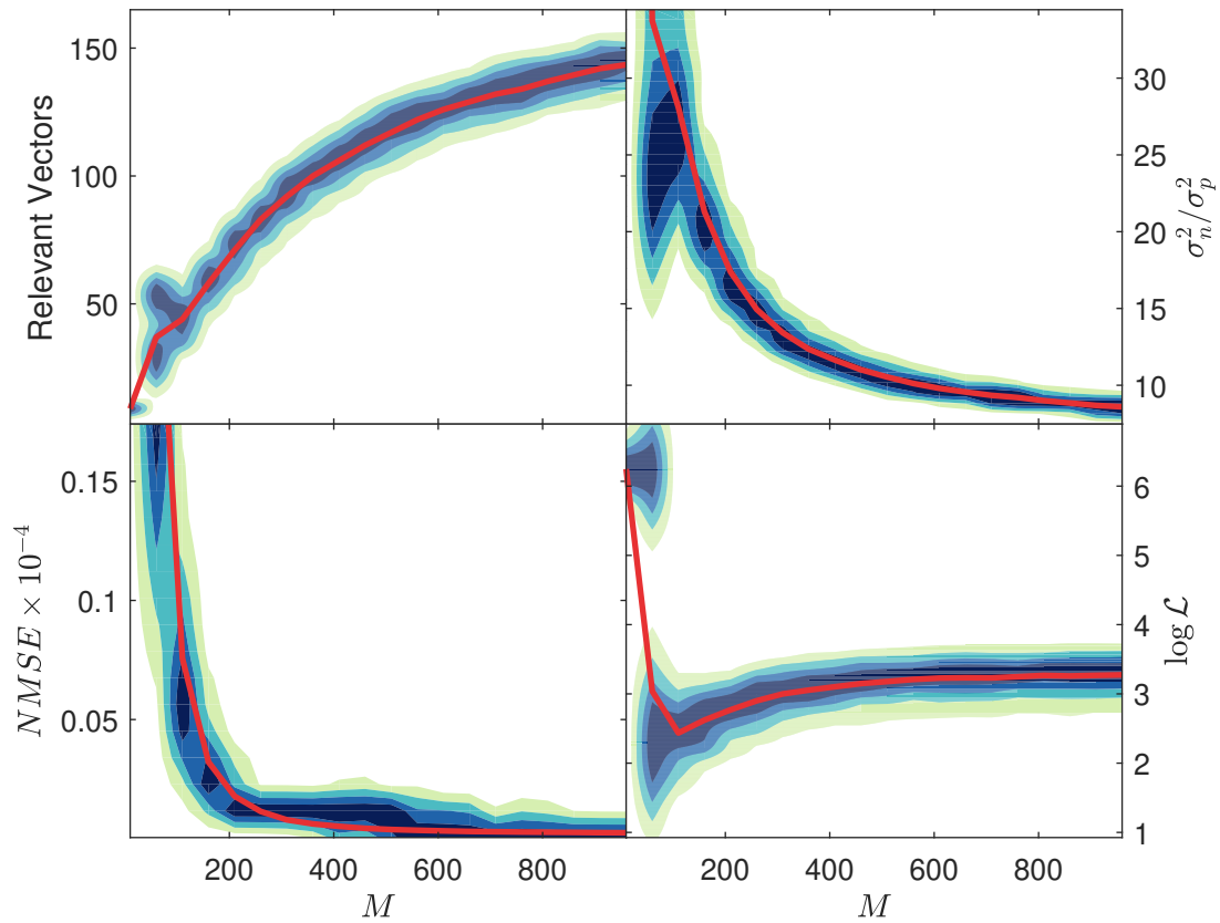
Figure 7: Compressed dimension, M against number of selected relevant vectors for 500 randomly selected ultrasound pulses from the C-scan data. The red line denotes the median, while the colour-map represents the density for the 500 draws.
