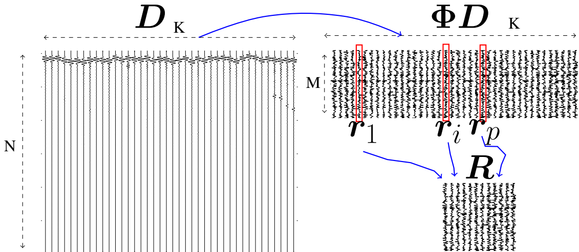
Figure 2: Illustration of application of random transform to a dictionary, and the selection of relevant vectors resulting from that transformation.
