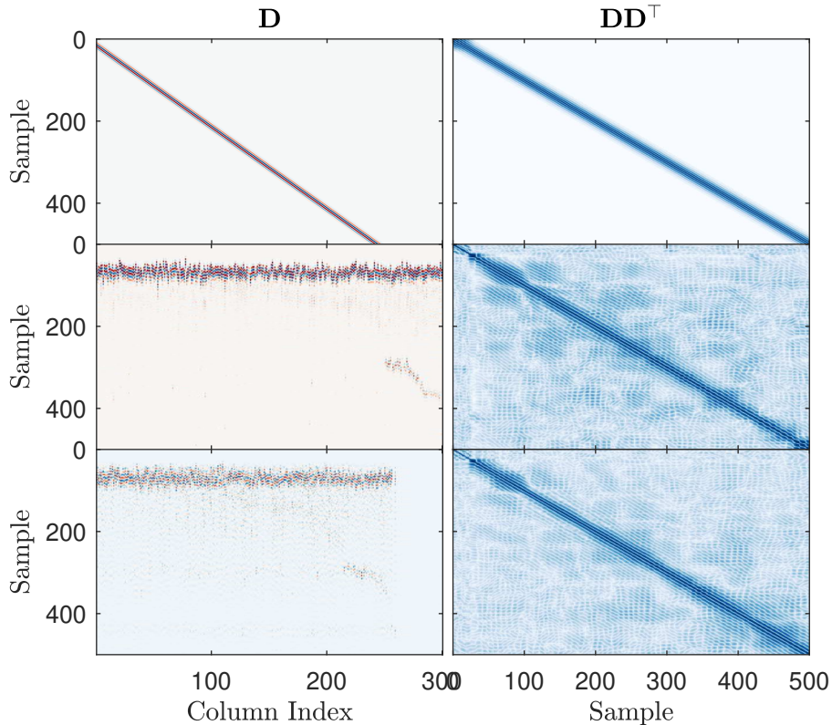
Figure 4: Comparison of three different dictionaries for the ultrasound data-set a) model-based tone-burst, b) k-means clustering and c) online matrix factorisation. The first column shows \mathbf{D} while the second column shows \mathbf{D}\mathbf{D}^\top
