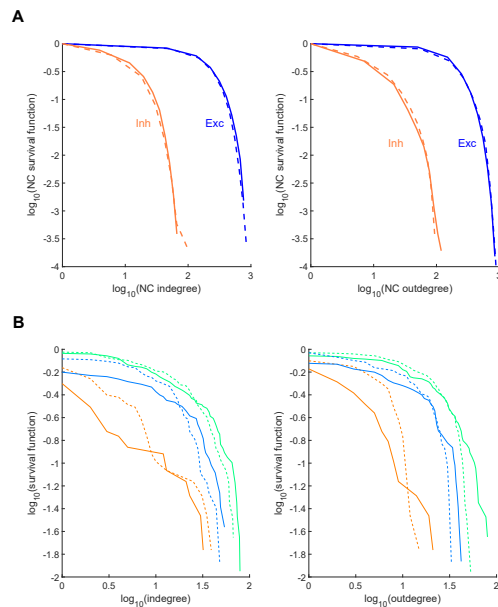
Figure 5: The new approach results in a quantitative agreement between model and data. A) Comparison between the survival functions of one of the NC datasets (solid lines) and our model (dotted lines) ( p < 0.025 for both the populations, with the Exc-Inh and Inh-Exc terms calculated from Kolmogorov-Smirnov distance). B) three representative experimental slices (solid lines) and three similar networks (dotted lines) extracted from the 5000 nodes network generated with our algorithm ( p < 0.1 for orange, blue, and green traces calculated comparing \gamma distributions of best fits).
