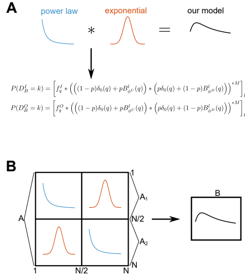
Figure 2: Schematic representation of the model. A) (top) schematic representation of the convolution process; (bottom) the equations describing the result of the convolution between the two original models to obtain the in- and out-degrees of the new model (see Suppl. Material for their derivation). B) Graphical illustration of the convolution process, which starts from the connectivity matrix of a network B and its blocks A_1 and A_2 . The final connectivity matrix B is calculated by considering the two power law blocks on the main diagonal and two exponential blocks in the antidiagonal of B as indicated in the diagram. Each subblock is a \frac{N}{2} \times \frac{N}{2} matrix.
