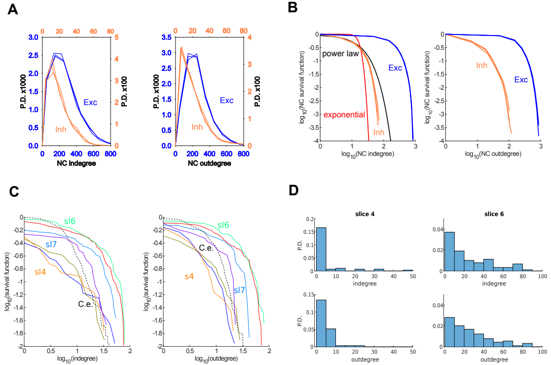
Figure 3: in- and out-degree from brain networks. A) Probability density of in- and out-degree for the excitatory (blue plots) and inhibitory (orange plots) neurons in three instances of the NC model network. Raw data were downloaded from ( https://bbp.epfl.ch/nmc-portal/downloads ) B) survival functions calculated from the plots in A); for comparison, the lines representing a power law (with degree distribution f_k = \frac{B(a+k, 2+\frac{a}{c})}{B(a, 1+\frac{a}{c})} with c = 17 and a = 100c ) and an exponential (with degree distribution g_k = \binom{N-1}{k} p^k (1-p)^{N-1-k} with p = 0.0033 and N = 5180 ) model are also shown. C) survival functions calculated from the data obtained in vitro in 7 slices (different line color) from neurons in the GABAergic CA3 region (from [33]). For comparison, the survival function obtained from the C. elegans network composed by all neurons connected through chemical synapses is also plotted (C.e., black dotted line, data taken and redrawn from [31]); the function for three slices are (sl4, sl6, and sl6) are explicitly indicated D) The in- and out-degree distribution for slice 4 and 6.
