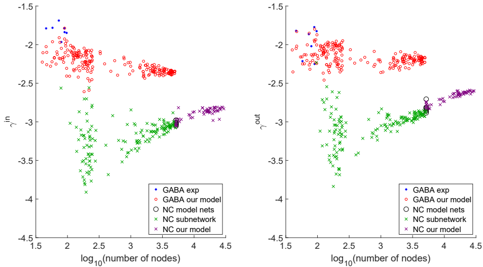
Figure 4: Large-scale network connectivity can be extrapolated by sampling a set of subnetworks. (Left) \gamma for the indegree distribution as a function of network size, in terms of number of nodes ( \log_{10} scale); Blue symbols represent the \gamma values calculated from the experimental data recorded from CA1 interneurons in 7 hippocampal slices; Red symbols represent the \gamma values for networks composed by different number of nodes, obtained by randomly sampling a 5,000-neurons network built with our model using parameters that best fit the experimental distributions. Black symbols are the \gamma values calculated from 7 instances of the approximately 5,000 neurons composing the NC inhibitory network. Green symbols represent the \gamma values obtained from smaller networks, randomly sampled from the 5,000-neuron network from [34]. Purple symbols represent our models projection for larger networks. (Right) same as in the left panel but for outdegrees.
