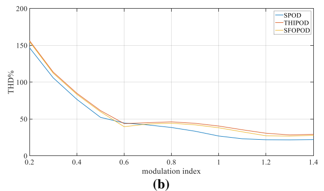
Fig. 15. Experimental results of the THD% for (a) line voltage and (b) phase voltage: SPOD, THIPOD and SFOPOD techniques.
