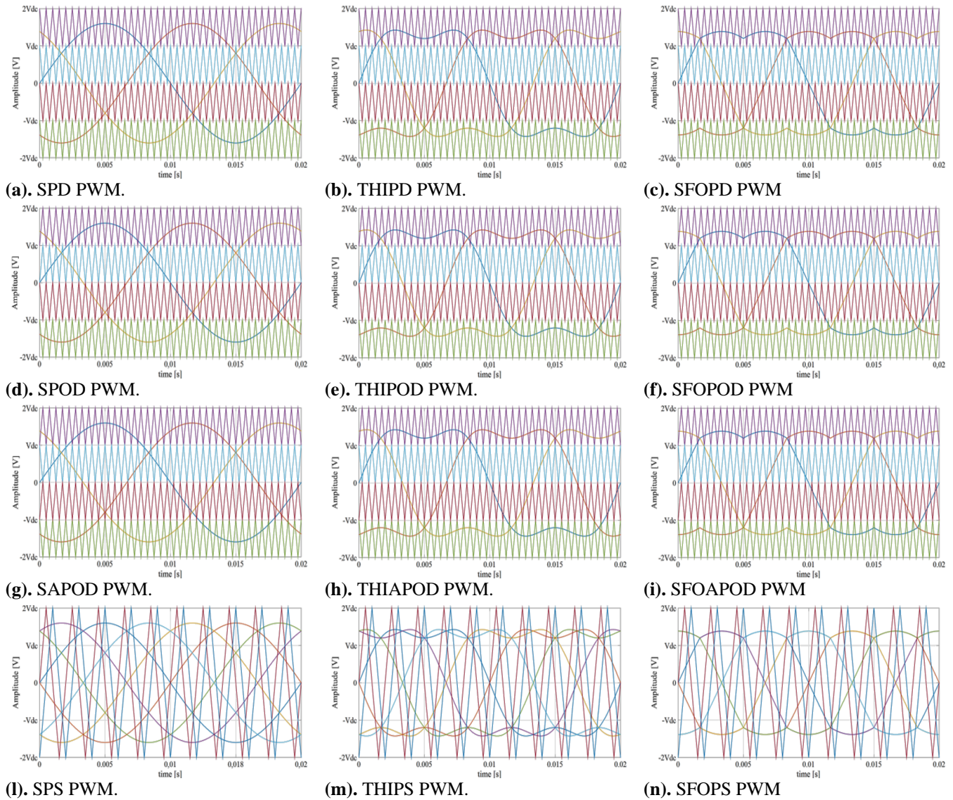
Fig. 4 (a-n). Graphical overview of the proposed modulation techniques.
