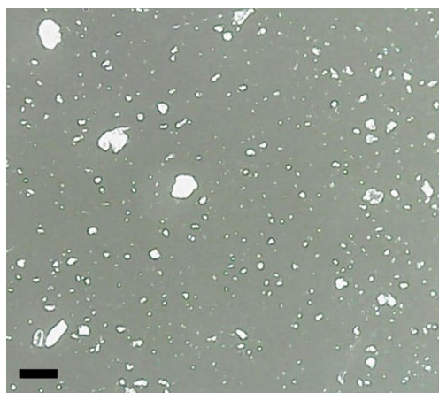
Fig. 7 Optical micrograph of talc- and particle-size distribution obtained by the analysis of 200 particles. Scale bar is 100 μm
