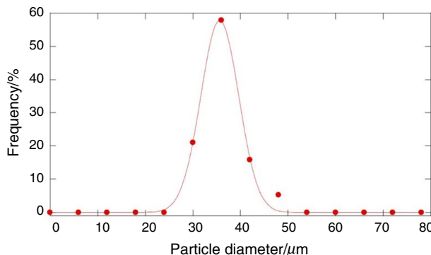
Fig. 7 Optical micrograph of talc- and particle-size distribution obtained by the analysis of 200 particles. Scale bar is 100 μm
