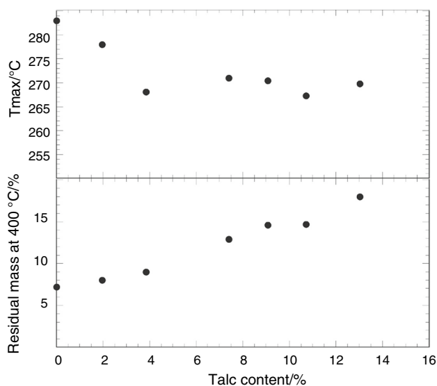
Fig. 2 Decomposition temperature ( T_{max} ) at the maximum of DTG and residual mass at 400 °C as a function of the talc content. Data refer to \beta = 5 °C min -1
