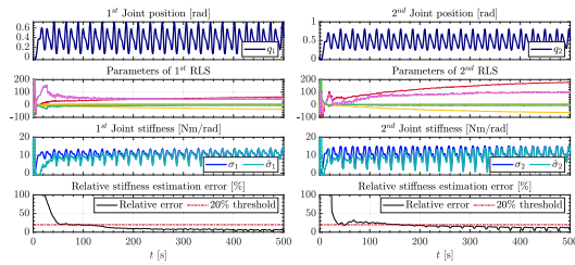
Fig. 7. Experiment #2 (2-DoF “A” setup). After an initial transient when Taylor’s coefficients are learned, the joint stiffness estimation errors, |\sigma_i - \hat{\sigma}_i|/\sigma_i , smoothly converge to within the 20%-threshold from the nominal value. The decentralized UIO+RLS-based solution successfully estimates the sought signal. The obtained performance indices, MSE and MSREP, evaluated after the transient ( t \in (300, 500) ), are, for the first joint, 0.5 \text{ N}^2 \text{ m}^2/\text{rad}^2 and 1% and, for the second one, 0.8 \text{ N}^2 \text{ m}^2/\text{rad}^2 and 4.8%, respectively.
