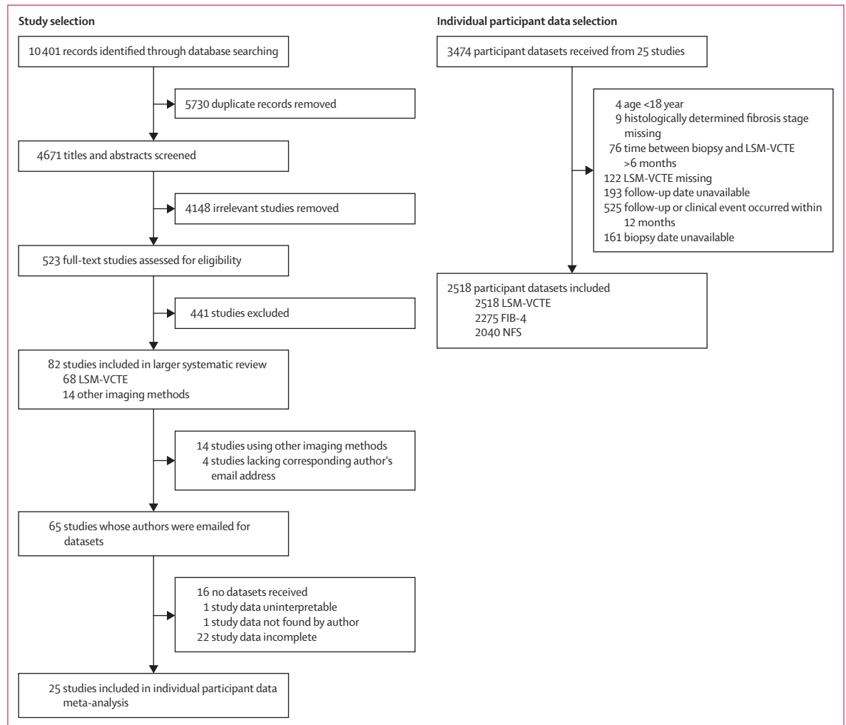
Figure 1: Study profile
