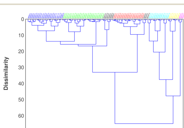
Fig. 8 Dendrogram of Ward's HCA clustering on the net area% dataset.
