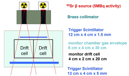
Figure 1: Schematic of the experimental set up of the monitoring drift chamber.
