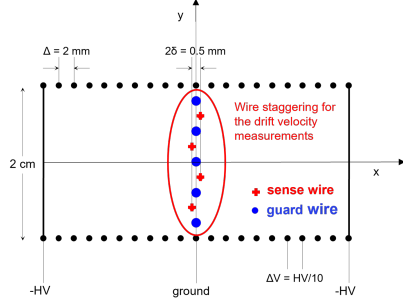
Figure 2: The transverse view of the monitoring drift chamber
