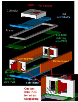
Figure 3: Mechanical design of the monitoring drift chamber
