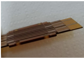
Figure 4: Custom PCB for wires staggering
