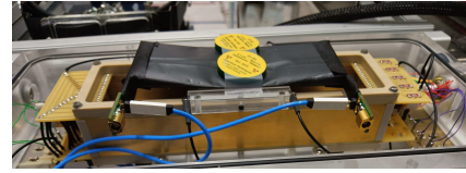
Figure 6: The two ^{90}\text{Sr} sources placed on top of the tapered scintillator.
