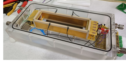
Figure 5: The monitoring drift chamber inside the gas box containment.
