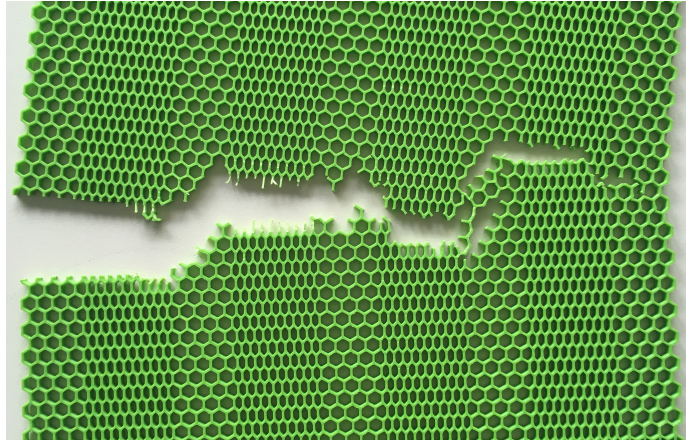
Fig. 6. Photographs showing the crack path for a gradient lattice structure made of ABS, from 5 .
