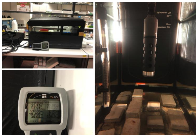
Fig. 3. Arrangement of experimental specimens inside the aquarium and monitoring system of seawater with the multiparametric probe
