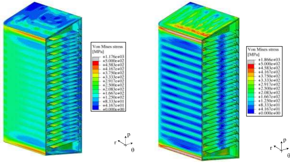
(a) NO Scenario (b) OP Scenario Fig. 3. TM results: Von Mises Stress Field
