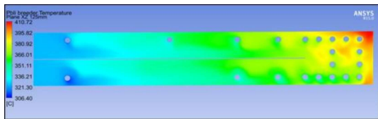
Fig. 4. Breeder temperature field by CFD code
