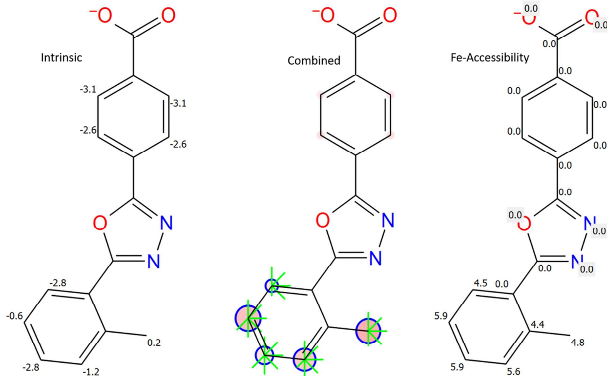
Figure 8. P450 site of metabolism (SOM). Intrinsic reactivity: positive values show high reactive site, negative values show weak reactive site; Fe-accessibility: positive values show high accessibility, negative values show poor accessibility, Combined reactivity: the number of rays indicates the values of the Fe-accessibility from IFD calculation, The circle encode 3 separate pieces of data. 1) the size of the circles indicates the overall SOM score – the larger the circle the better the score, 2) the color of the circle indicates the atomic intrinsic reactivity – the redder the circle, the higher the intrinsic reactivity, 3) a blue ring around the circle indicates that the atom passed through the CYP filtering stage.
