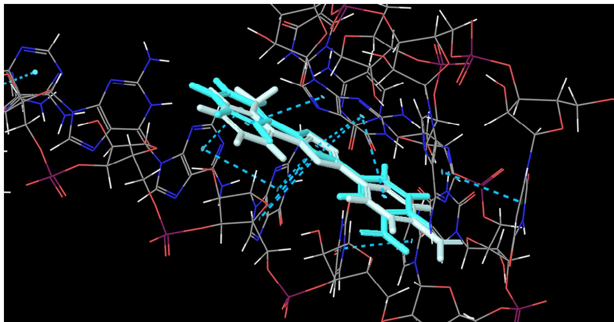
Figure 6. IFD poses of NV2445 (light blue) compared with PTC124 equilibrium pose (grey). Dashed light blue lines represent the \pi - \pi stacking interaction.
