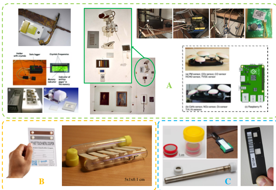
Fig. 4. Visual impact comparison between on-line (A – most utilized methods that rely on electricity) and off-line (B – here discussed bi-metallic Purafil™ and marble coupons – and C – other available types of comparable off-line methods) sensors.
