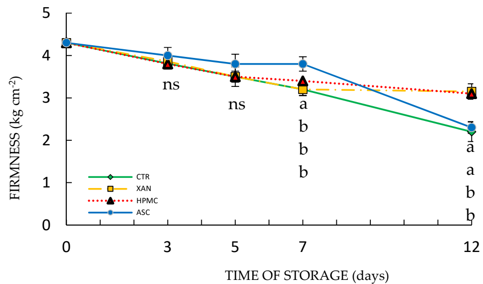
Figure 2. Development of firmness ( \text{kg cm}^{-2} ) of treated (XAN, HPMC, ASC) and untreated fresh-cut slices of Pyrus communis L. pear (Abate Fétel) just after cut (0) and at 3, 5, 7, 12 days of storage at 4 °C. At each sampling date, different letters indicate substantial changes between treatments. At each sampling date, ns indicate no changes between treatments. p \leq 0.05 was used in the Tukey's test. The data are provided as the mean \pm S.E. ( n = 3 ).
