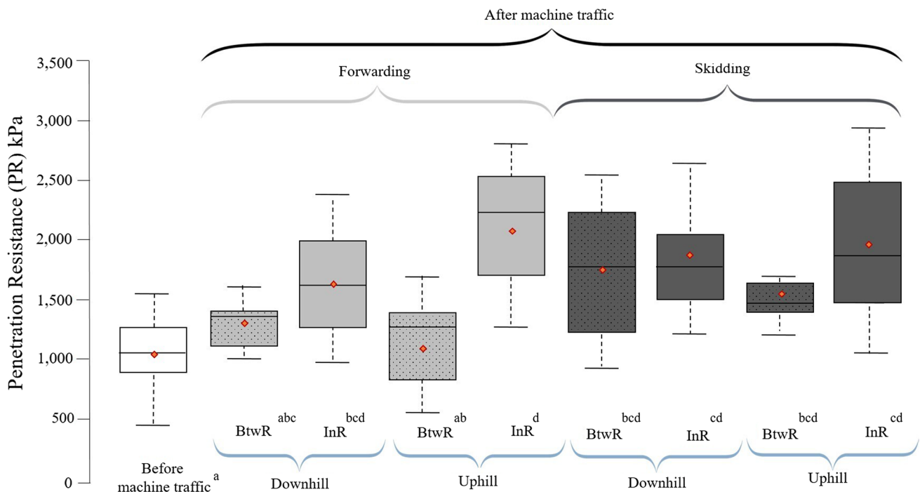
Fig. 6 Average values of penetration resistance (red diamonds) after 127 m 3 of wood passed on the trails (including median and spreading range) by 10 and 45 passes for skidding and forwarding, respectively. Data about driving direction (uphill or downhill) and sam-
