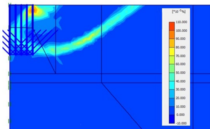
Figure 5. Incremental shear strain at failure for the case of a homogeneous soil foundation made of sand with \phi' = 35^\circ and \psi' = \phi' ( B = 1 m).
