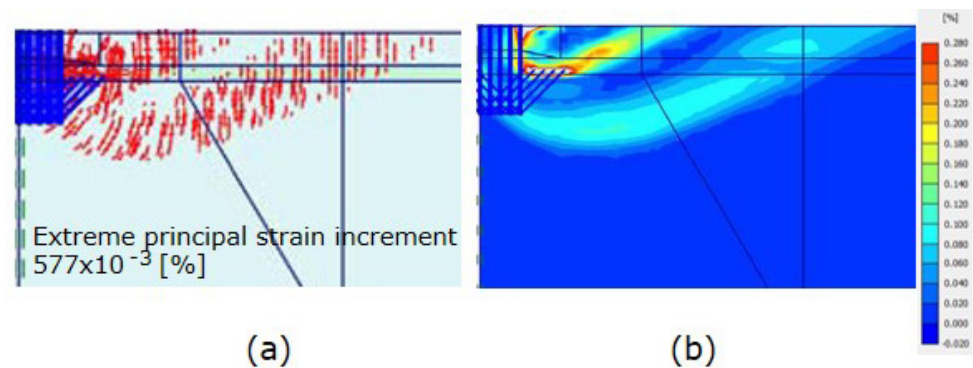
Figure 12. Incremental strains for the case in which the sand has \varphi'_1 = 40^\circ and \psi'_1 = 40 while the weak layer is characterised by \varphi'_2 = 30^\circ and \psi'_2 = 30 ; the depth of the weak layer is z_i/B = 0.5 . (a) principal directions; (b) shear shadings.
