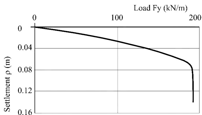
Figure 4. The load-settlement curve for foundation soil made of sand with \phi' = 35^\circ , \psi' = \phi' , and B = 1 m.
