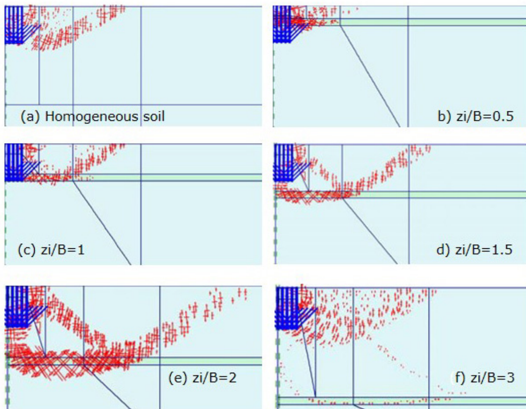
Figure 9. Incremental strains (principal directions) at failure for \phi'_1 = 40^\circ , \psi'_1 = 2/3\phi'_1 = 26.7^\circ (sand), \phi'_2 = 15^\circ , \psi'_2 = 0 (weak layer), as a function of the relative depth z_i/B of the weak layer ( B = 1 m).
