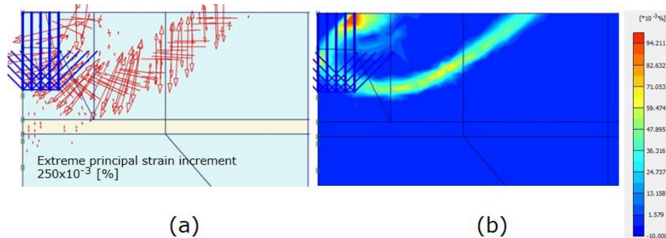
Figure 8. Incremental strains at failure for the case in which the sand has \phi'_1 = 40^\circ and \psi'_1 = 40^\circ , while the weak layer is characterised by \phi'_2 = 35^\circ and \psi'_2 = 35^\circ ; the depth of the weak layer is z_i/B = 1.5 . (a) principal directions; (b) shear shadings.
