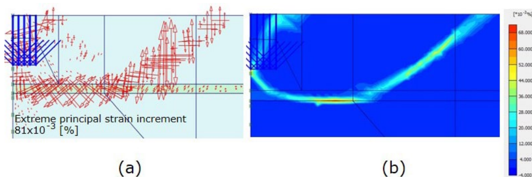
Figure 7. Incremental strains at failure for the case in which the sand has \phi'_1 = 40^\circ and \psi'_1 = 15^\circ , while the weak layer is characterised by \phi'_2 = 10^\circ and \psi'_2 = 0 ; the depth of the weak layer is z_i/B = 1.5 . (a) principal directions; (b) shear shadings.
