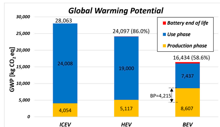
Figure 1. Global warming potential related to the entire lifecycle of the three reference vehicles (BP = Battery Production).
