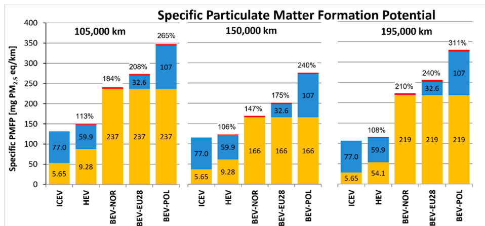
Figure 9. Specific particulate matter formation potential (mgPM 2.5 eq/km) related to the three reference vehicles in the six different scenarios.
