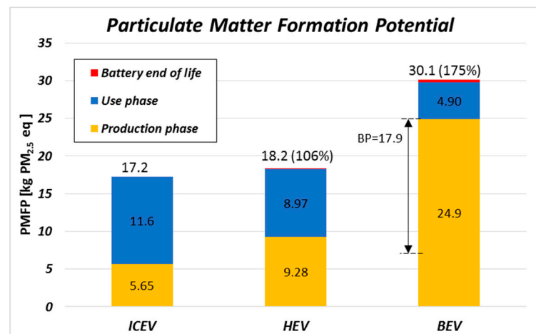
Figure 4. Particulate matter formation related to the entire lifecycle of the three reference vehicles (BP = Battery Production).
