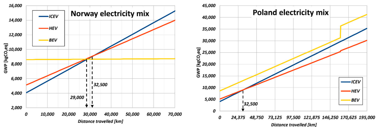
Figure 12. Global warming impacts comparison as function of the lifetime traveled distance, with reference to the Norwegian (left) and to the Polish (right) electricity mix.
