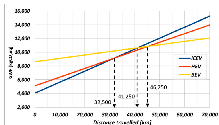
Figure 2. Global warming potential comparison as a function of the lifetime distance traveled.
