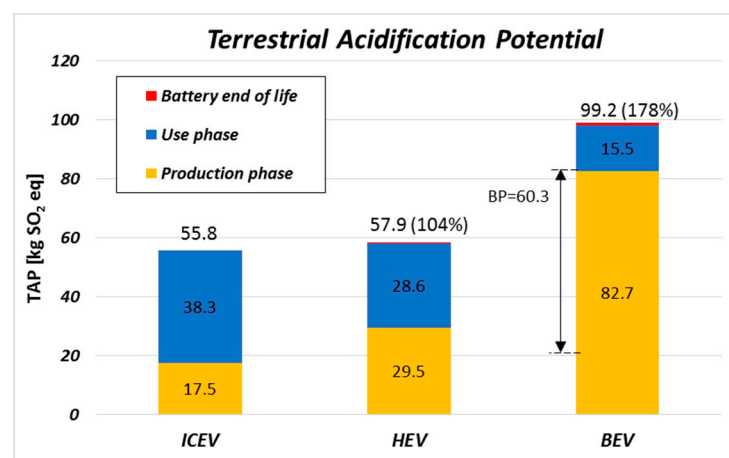
Figure 3. Terrestrial acidification caused during the entire lifecycle of the three reference vehicles (BP = Battery Production).
