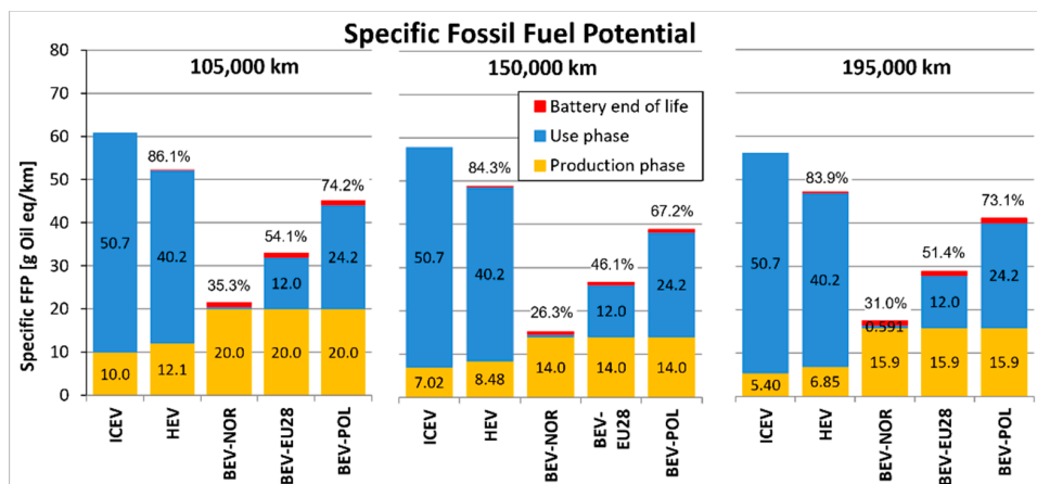
Figure 11. Specific fossil fuel potential (gOil-eq/km) related to the three reference vehicles in the six different scenarios.
