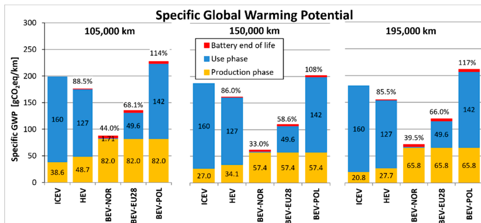
Figure 7. Specific global warming potential (gCO 2 eq/km) related to the three reference vehicles in the scenario analysis.
