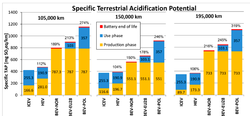
Figure 8. Specific terrestrial acidification potential (mgSO 2 eq/km) related to the three reference vehicles in the scenario analysis.
