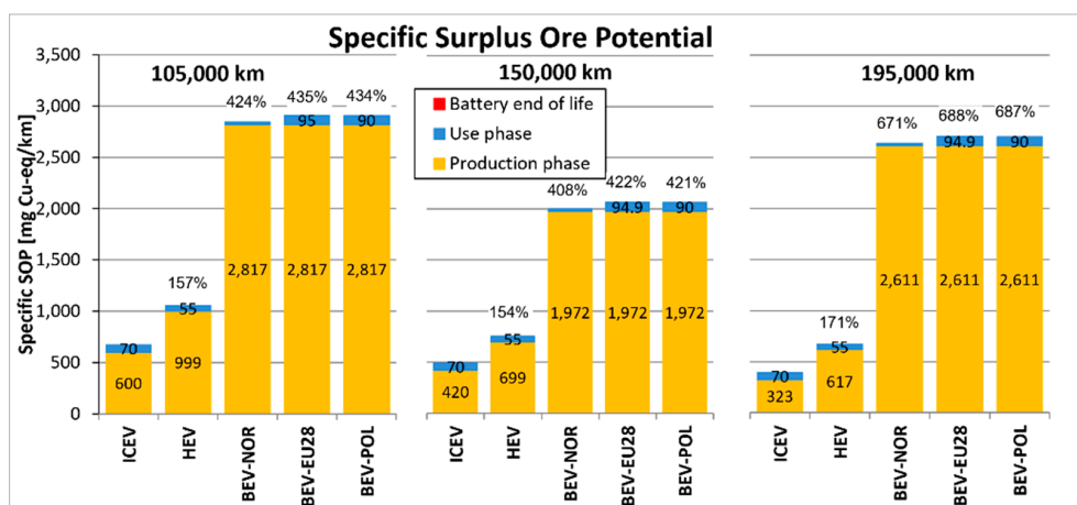
Figure 10. Specific surplus ore potential (mgCu-eq/km) related to the three reference vehicles in the six different scenarios.
