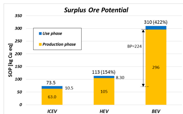
Figure 5. Mineral resource depletion related to the entire lifecycle of the three reference vehicles (BP = Battery Production).
