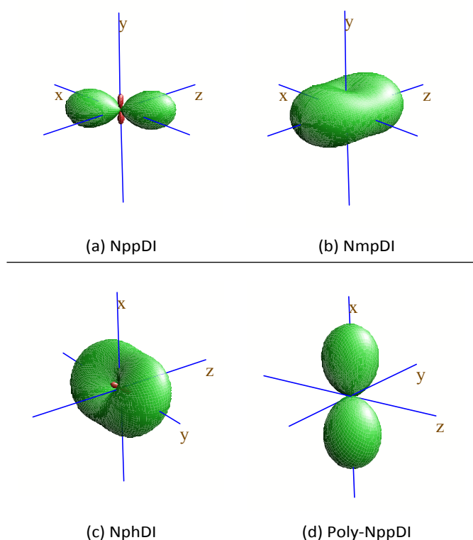
Figure 6. Visualization of the thermal expansion tensors, calculated by comparing lattice metrics at RT and at 300°C. Positive lobes in green, (tiny) negative ones in red.
