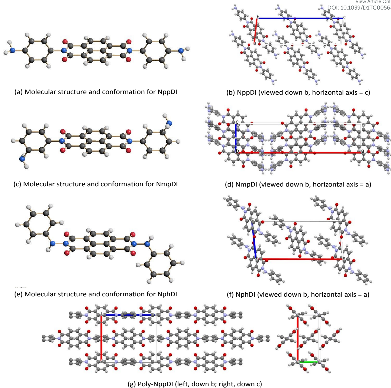
Figure 2. Schematic drawings of the molecular structure and crystal packings of (a,b) NppDI, (c,d) NMPDI and (e,f) NphDI, together with a note of their orientations. In g), the polymeric Poly-NppDI structure is shown. Color codes: C in grey, N in blue, O in red and H in white. Graphics realized by Schakal 42 (a,c,e) and Mercury 43 (b,d,f,g).
