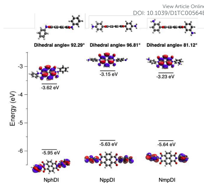
Figure 8. Energy scheme and HOMO and LUMO isosurfaces for NphDI, NppDI, and NmpDI (left to right).
