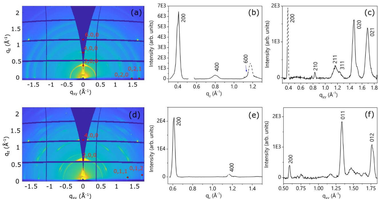
Figure 9. 2D-GIXD images of annealed (a) NmpDI and (d) NphDI thin films recorded for \alpha_i = 0.1^\circ . The corresponding integrated intensity profiles along q_z , [(b) and (e)], and along q_{xy} , [(c) and (f)] are reported. The dashed lines in (b), (c), and (e) are Gaussian fits to the experimental data at the positions where the detector cuts hamper collection of the diffracted intensity.
