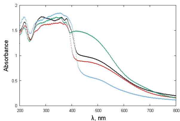
Figure 7. Absorbance spectra (in the form of F[R(E)] through Kubelka-Munk transformation of the diffuse reflectance spectra) of NppDI (black), NmpDI (red), NphDI (green) and Poly-NppDI (blue).
