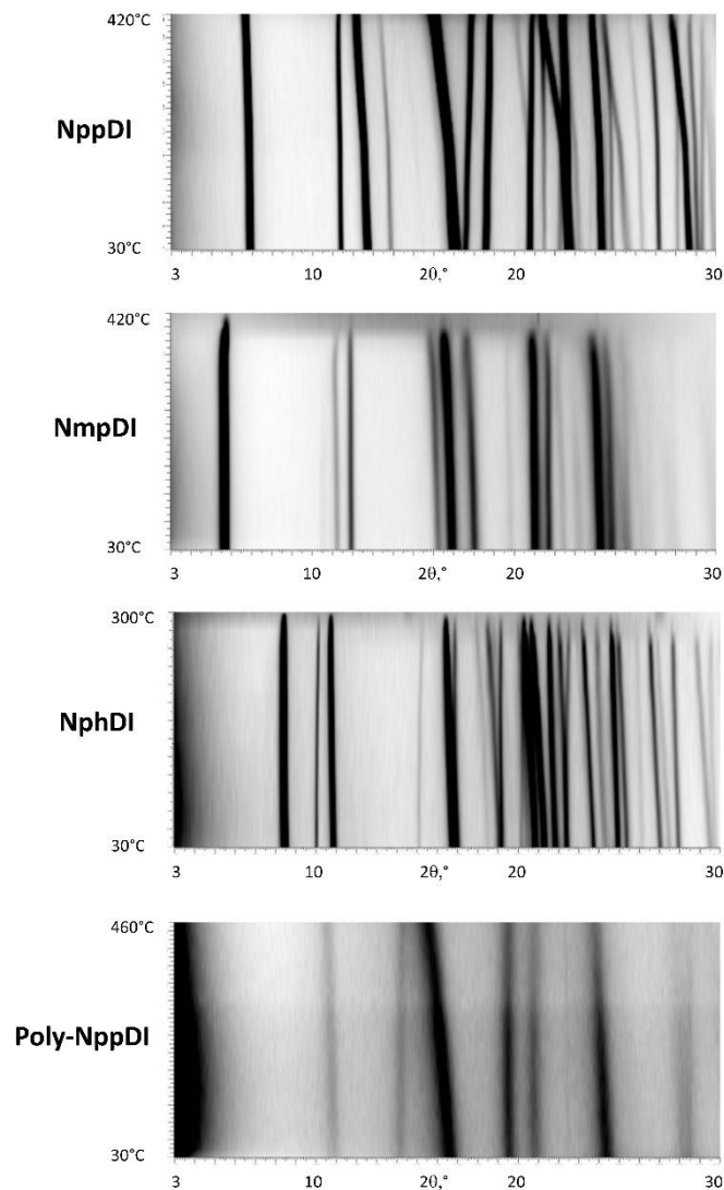
Figure 5. Variable temperature XRD scans ( 2\theta in the 3-30° range), from RT (bottom) to 420, 420, 300, 460°C, respectively
