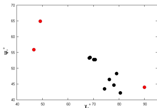
Figure 3. Stereochemical descriptors \chi, \psi for the \pi - \pi stacking of the crystal phases of this work (red dots, values from Table 2) and the aliphatic analogues (black dots) reported in ref. 9.
