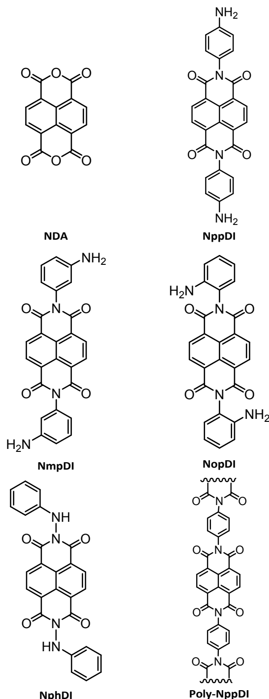
Chart I. Molecular sketches and labeling of the species discussed in this work.
