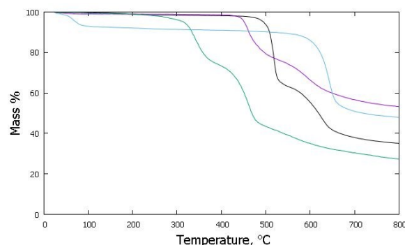
Figure 4. TG traces collected under N 2 at a scan rate of 10° min -1 : NppDI in black; NmdPI in magenta; NphDI in green; Poly-NppDI in blue.
