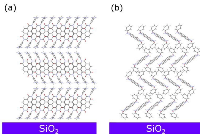
Figure 10: Sketch of the dominant molecular arrangement of the (a) NmpDI and (b) NphDI thin films on the substrate surface, as retrieved from GIXD analysis.
