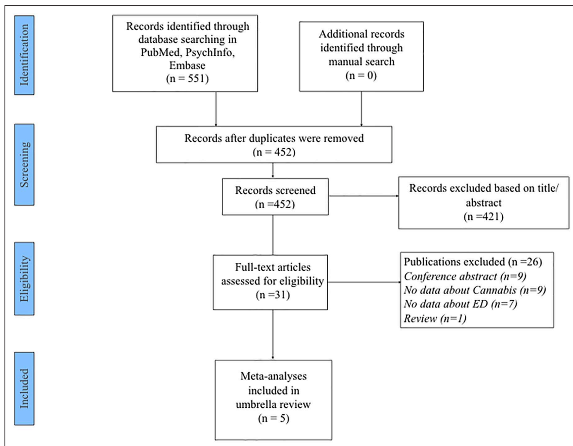
Figure 1. PRISMA flow-chart.
