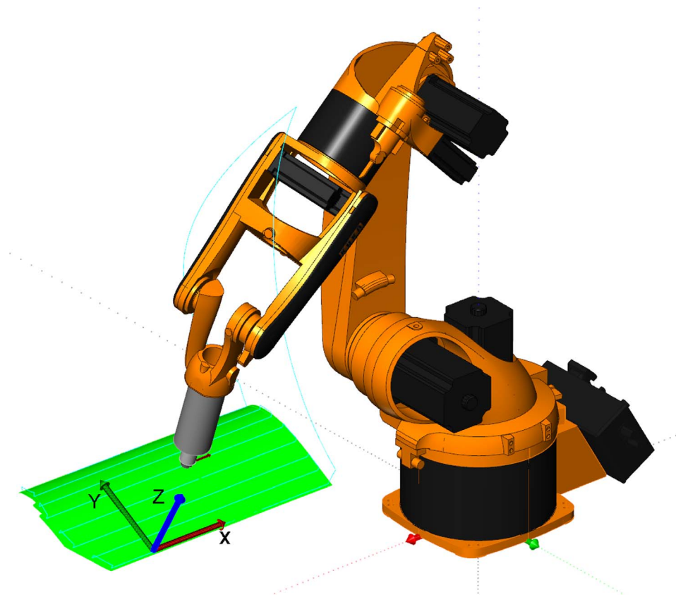
Fig. 3. Simulated robotic NDT scan environment showing robotic arm in orange, test piece (leading edge skin) in green, scan path in turquoise, NDT probe and its holder in grey, base reference coordinate frame (arrows). (For interpretation of the references to colour in this figure legend, the reader is referred to the web version of this article.)
