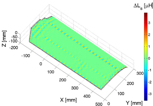
Fig. 6. CAD overlay of EC inductance change during robotic scan of the edge skin at 400 kHz.
