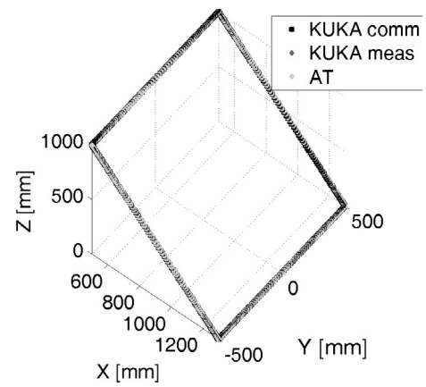
Fig. 8. Shape of the test path as measured at 100% rated speed showing command coordinates and actual coordinates reported by the robot's encoders as well as the transformed coordinates measured with the laser tracker.
