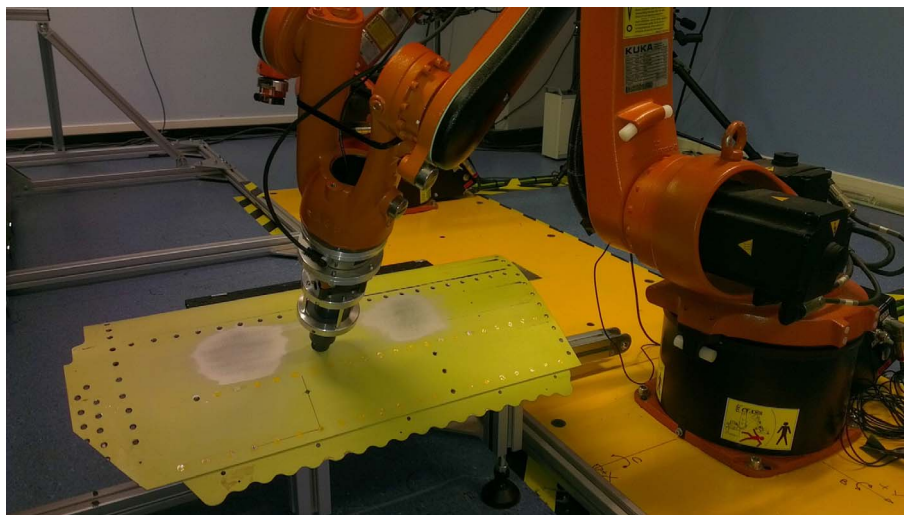
Fig. 4. Illustration of practical implementation of the generated scan path for NDT of a fixed leading edge skin panel by means of KUKA KR5 arc HW robot.
