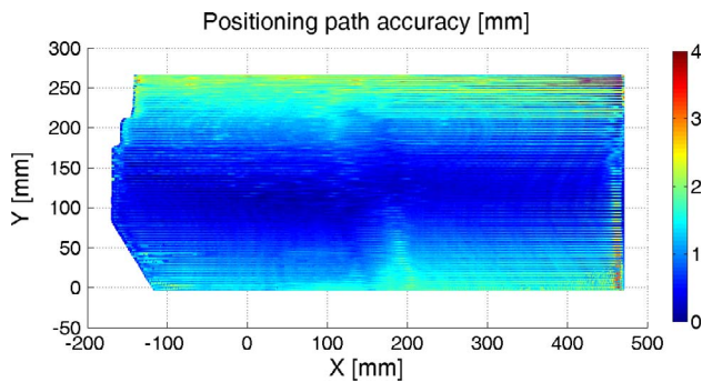
Fig. 9. Positional error measured along the generated NDT scan path at 100% rated speed.
