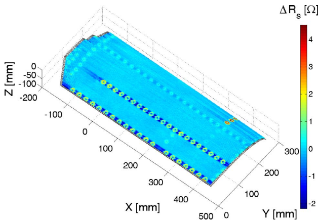
Fig. 5. CAD overlay of EC resistance change during robotic scan of the edge skin at 400 kHz.
