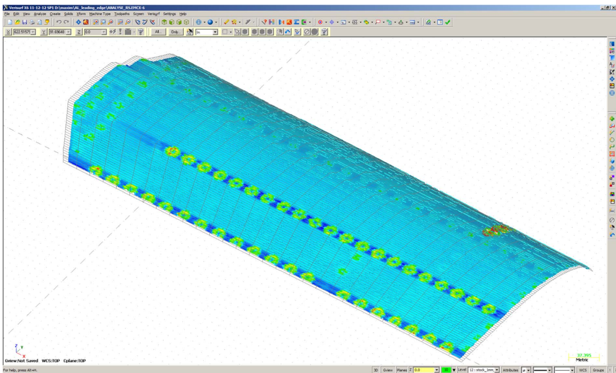
Fig. 7. Overlay of NDT response at 400 kHz on CAD model in Verisurf metrology software.
