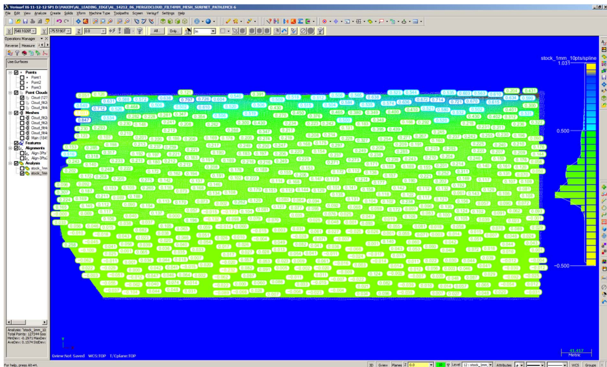
Fig. 2. Accuracy map of the reverse engineered leading edge skin.
