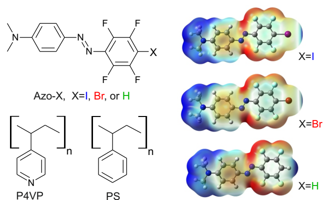
Fig. 1 Chemical structures of the components used in the studied material systems (left) and M062X/6-311++G(d,p) MEP maps (right). Potentials are mapped on the respective isosurfaces (0.001 a.u.) of electron density. Values of electrostatic potential range from -0.03 (red) to 0.03 (blue) a.u., with most positive local values on X equal to 0.037, 0.033 and 0.041 a.u. for X=I, Br and H, respectively. Atom color scheme: C, gray; H, light gray; N, dark blue; Br, red; F, sky blue, I, magenta.
