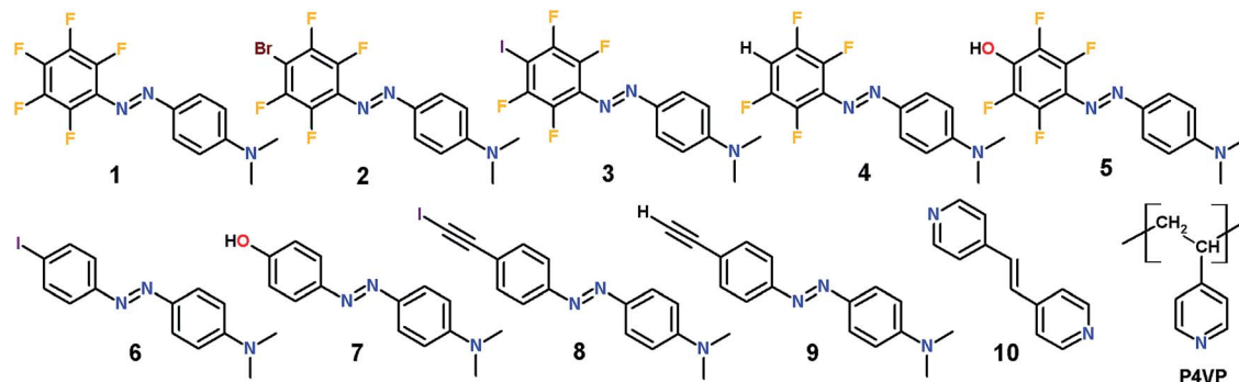
Fig. 1 Chemical structures of fluorinated azobenzene modules 1–5, hydrogenated azobenzene modules 6–9, model dipyrindyl compound 10 used in the co-crystallization studies, and poly(4-vinyl pyridine) (P4VP) that was used as the polymer matrix for the azobenzene dyes.
