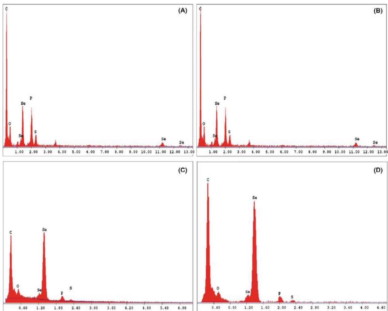
Fig. 3. Energy-dispersive X-ray spectroscopy (EDX) spectra of Bio Se-NEMO-S produced by Bacillus mycoides SeITE01 after 6 (A) or 24 h (B) of \text{Na}_2\text{SeO}_3 exposure, and chemical SeNPs made using L-cysteine (C) or ascorbic Acid (D).
