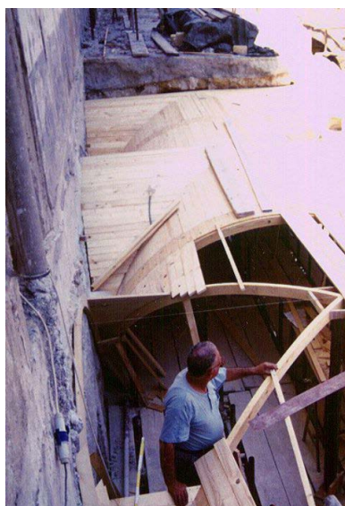
Figures 10, 11. Ribs of wooden centering and view of continuous intrados of the same supporting framework.
