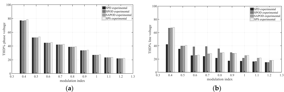
Figure 10. Comparison between the experimental THD% results for (a) phase voltage and (b) line voltage.
