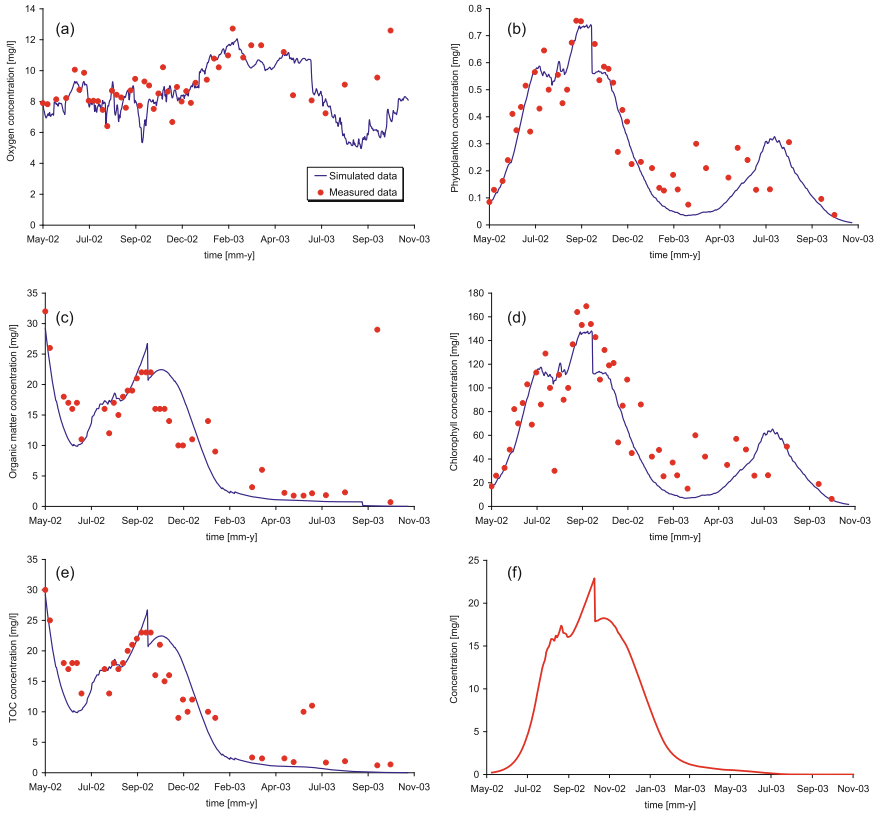
Fig. 2. Model results in terms of: oxygen concentration (a); phytoplankton(b); organic matter (c); chlorophyll (d); TOC (e) and zooplankton (f)
