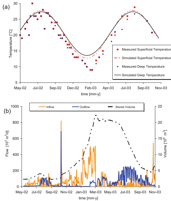
Fig. 1. Temperature profiles (a); water budget balance (b)
