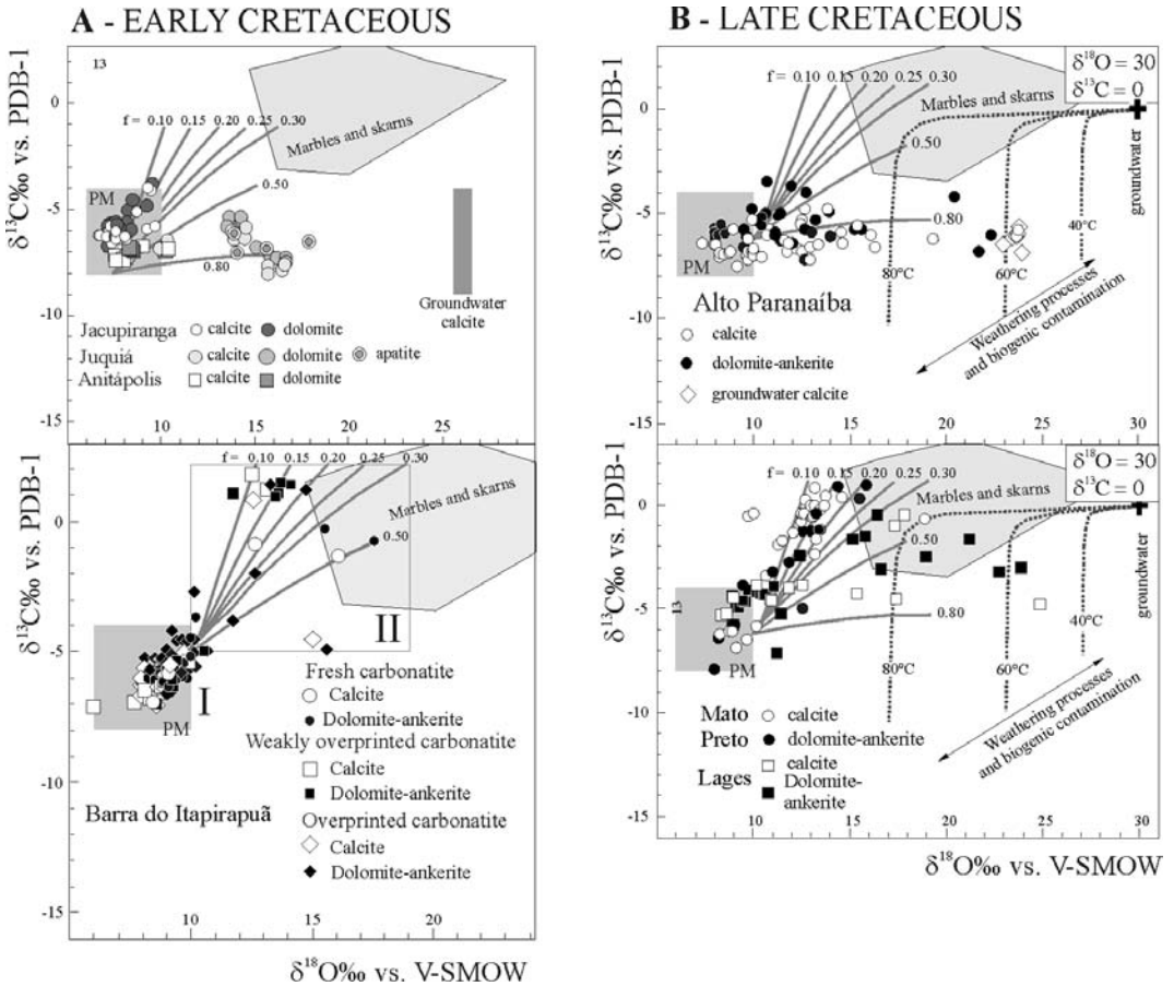
Fig. 13 – Plot of \delta^{18}\text{O} vs. \delta^{13}\text{C} for the carbonatite samples from Early Cretaceous (A: Jacupiranga, Juquiá, Anitápolis; Barra do Itaipirapuã) and Late Cretaceous complexes (B: Alto Paranaíba, Mato Preto and Lages), compared with the results from the proposed model ( f = [(A-b)/A] ; I, magmatic evolution; II, fluid-related hydrothermal recrystallization; see text). Data for Meso- and Neoproterozoic marbles and skarns after Mello and Bettencourt (1998); groundwater calcite, after Alcover et al
