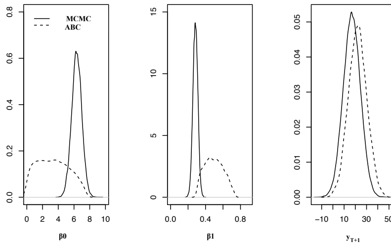
Fig. 2 Marginal posteriors for the parameters, both considering the MCMC and ABC methods for the monthly time series of Aipe river basin (on the left and in the middle). Predictive density functions both MCMC and ABC (on the right).
