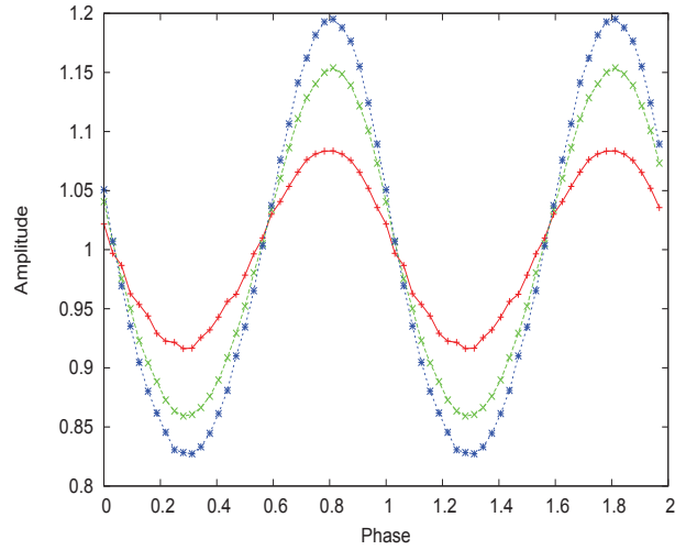
Figure 4. Top panel: energy-averaged pulse-folded profile (32 channels) and best-fitting model using two sinusoids. Bottom panel: pulse-folded profile for the EPIC/pn data in energy bands: 0.5–3.0 keV (red data), 3.0–6.0 keV (green data), and 6.0–12.0 keV (blue data).
