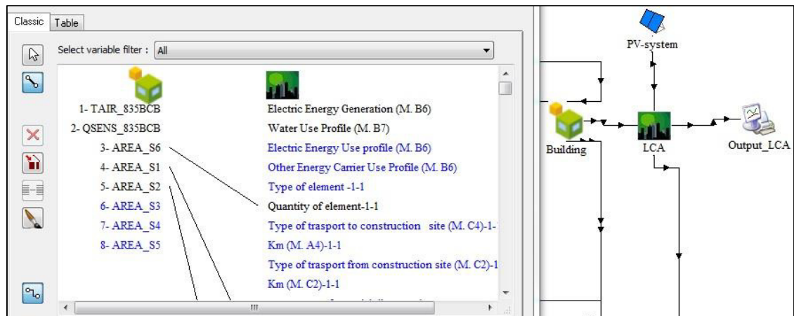
Fig. 3. Connection of Type 56 (on the left) to the LCA Type (on the right) in TRNSYS – Simulation Studio.
