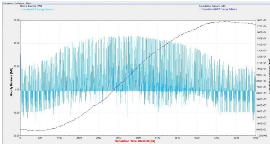
Fig. 4. Net Zero Energy Balance results output.
