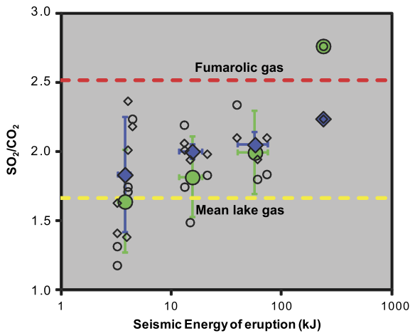
Fig. 3. Relationship between SE and \text{SO}_2/\text{CO}_2 . Diamonds are the average \text{SO}_2/\text{CO}_2 recorded within 24 h of eruption and circles indicate the closest \text{SO}_2/\text{CO}_2 value measured before each eruption. The individual eruptions (open symbols) naturally fall into four categories (closed symbols) based on seismic energy: \text{SE} < 10 ; 10 < \text{SE} < 30 ; 30 < \text{SE} < 150 ; \text{SE} > 150 . Small eruptions on average are associated with lower \text{SO}_2/\text{CO}_2 and display high variance, whereas large eruptions show high associated \text{SO}_2/\text{CO}_2 , closest to fumarolic gas. This relationship is maintained considering only precursory gas measurements (green filled circles) and the generally lower \text{SO}_2/\text{CO}_2 values observed before eruptions reflect the fact that eruptions tend to occur before the peak in \text{SO}_2/\text{CO}_2 (Fig. 2). (For interpretation of the references to color in this figure legend, the reader is referred to the web version of this article.)
