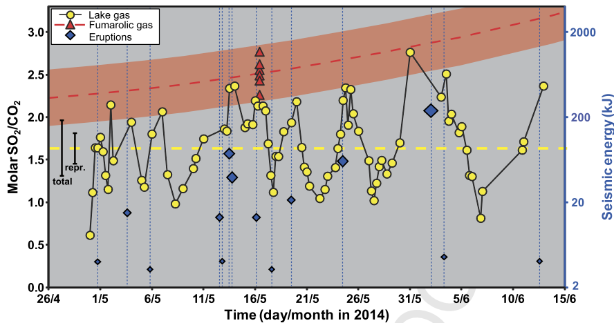
Fig. 2. Time series lake gas \text{SO}_2/\text{CO}_2 and SE of eruptions. The yellow dashed line is the median of lake gas \text{SO}_2/\text{CO}_2 (1.64). Total error in Multi-GAS measurements is conservatively estimated at 20% from experimental results ( \pm 0.33 for \text{SO}_2/\text{CO}_2 of 1.64; see Methods), whereas the average reproducibility of the lake gas measurements is 0.18 (error bars shown at left). The composition of the dome fumaroles was measured on 16 May, and the fumarolic compositional trend is constrained by Multi-GAS campaigns between January and July of 2014 (Fig. S3). The sizes of the blue diamonds correspond to phreatic eruption groups as defined by SE (Fig. 3). (For interpretation of the references to color in this figure legend, the reader is referred to the web version of this article.)
