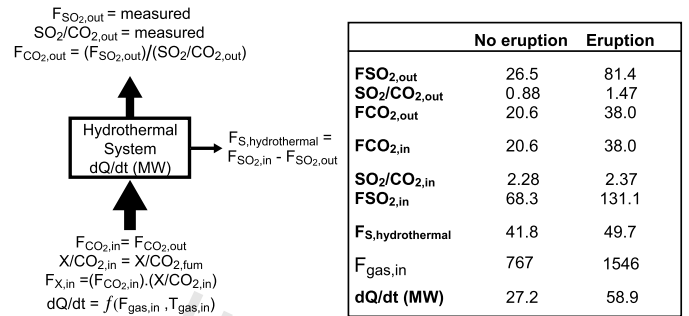
Fig. 6. Box model for gas inputs and outputs for the Poás hydrothermal system (see Table 2). The SO 2 flux from the system (FSO 2,out ; all fluxes in units of T/day) and SO 2 /CO 2,out are constrained by DOAS and Multi-GAS measurements, respectively, allowing calculation of the CO 2 flux from the lake (FCO 2,out ). The CO 2 flux from the lake is equal to the CO 2 flux into the lake (FCO 2,in ) because CO 2 is inert in acidic fluids. The composition of gas feeding the lake is constrained by gas ratios measured at the high temperature fumaroles (X/CO 2,fum ; where X = H 2 O, SO 2 , H 2 S, and H 2 ), which allows calculation of the flux of gases into the crater lake (F X,in ) and the flux of S lost to the hydrothermal system (F s,hydrothermal ; expressed in T/d SO 2 ). As the flux and composition of magmatic gas into the lake are constrained, the heat transfer to the crater lake (dQ/dt) can be quantified (see supplementary online text for calculation details).
