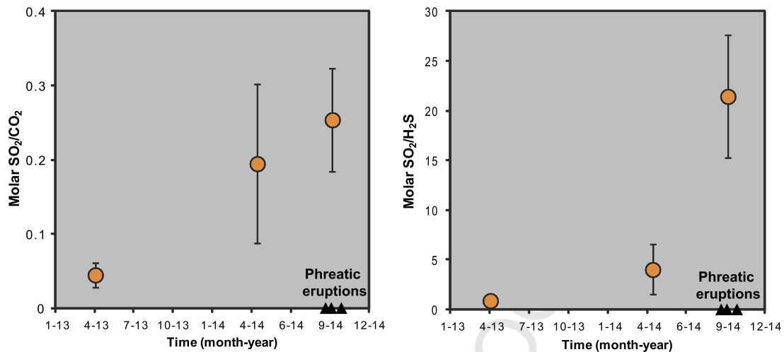
Fig. 7. Results of Multi-GAS campaigns conducted at Rincón de la Vieja volcano (Northern Costa Rica), which also hosts an ultra-acid crater lake. Data for April 2013 from Galle et al. (2002). Seismically registered phreatic eruptions occurred in September and October of 2014 and were associated with significant increase in SO 2 /CO 2 and SO 2 /H 2 S.
