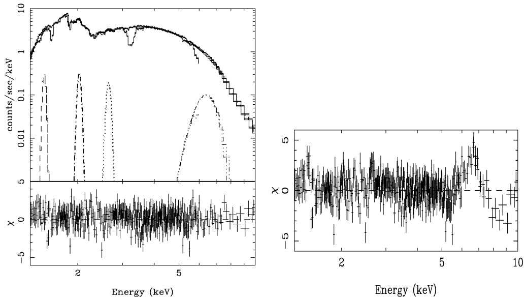
Fig. 2 Left: Top panel: HEG first order spectra of 4U 1705–44 together with the best-fit model (see Table 2). The discrete features included in the best-fit model and described by Gaussians are also shown. Bottom panel: Residuals in units of \sigma with respect to the best-fit model. Right: Residuals in units of \sigma with respect to the simple Comptonization continuum when the iron line and other low energy Gaussians are not included in the model.
