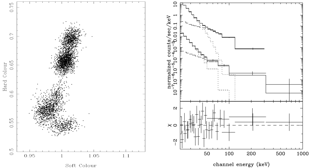
Fig. 1 Left: Color-color diagram of Sco X-1 from PCA data during the simultaneous INTEGRAL/RXTE observation. Here Soft Color is the ratio of the count rate in the energy bands [3.5 - 6 \text{ keV}]/[2 - 3.5 \text{ keV}] and Hard Color is the ratio [9.7 - 16 \text{ keV}]/[6 - 9.7 \text{ keV}] , respectively. Only data from PCUs 2 and 3, which were on for most of the observation, have been used. The four colors indicate the four regions in which the CD has been divided and from which INTEGRAL spectra were extracted. Right: Top: ISGRI (20–200 keV, black) and SPI (20 keV–1 MeV, red) data of Sco X-1 together with the best-fit model (solid lines on top of the data) composed of the Comptonization model ( \text{comptt} , dotted lines) and a cutoff power law (dashed lines). Bottom: residuals in units of \sigma with respect to the best-fit model.
