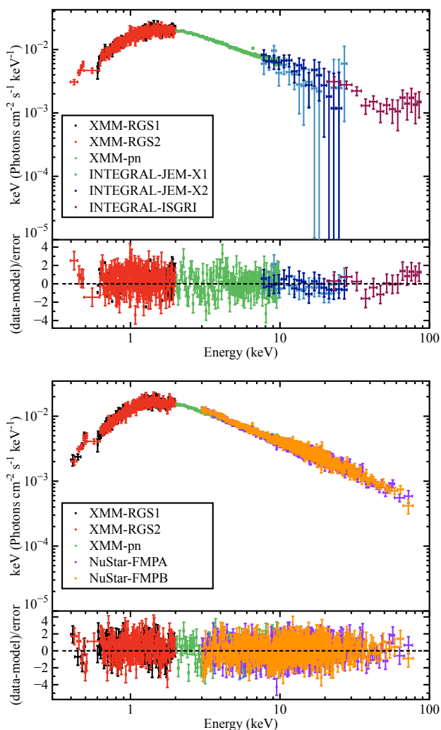
Fig. 4. Top panel - Broad-band (0.4–100 keV) energy spectrum of Obs.1 including XMM-Newton RGS1 (black), RGS2 (red) and PN (green) and INTEGRAL JEM-X (blue and cyan) and IBIS/ISGRI . Bottom panel - Broad-band (0.4–80 keV) energy spectrum of Obs.2 including XMM-Newton RGS1 (black), RGS2 (red) and PN (green) and NuSTAR FMPA/B (orange and violet). For both energy spectra the residuals with respect to the best fit models are given in units of \sigma .
