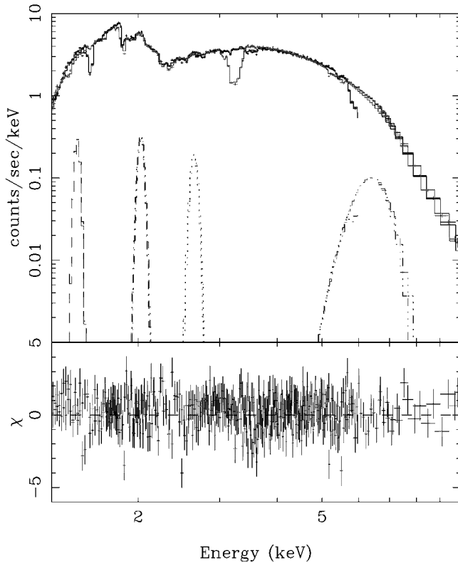
FIG. 1.— Top panel : HEG first-order spectra of 4U 1705–44 together with the best-fit model (see Table 1). The discrete features included in the best-fit model and described by Gaussians are also shown. Note that, for the sake of clarity, we have rebinned the data in the plot with respect to the energy resolution used for the spectral analysis. Bottom panel : Residuals in units of \sigma with respect to the best-fit model. [See the electronic edition of the Journal for a color version of this figure.]
