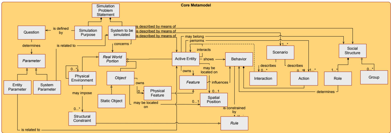
Fig. 4. The Core Metamodel derived from the domain under analysis.
