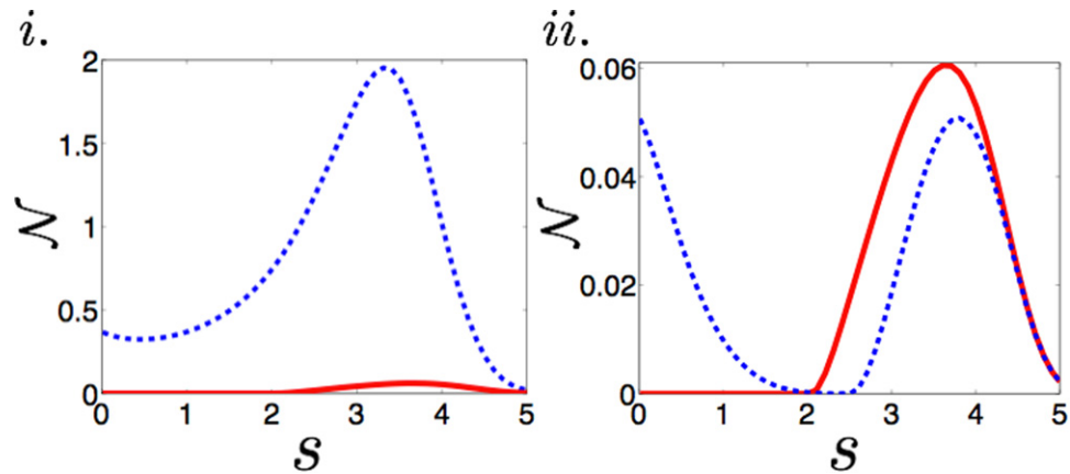
Figure 4. Non-Markovianity measure against the Ohmicity parameter s for the dynamically decoupled system (blue dotted line) for time intervals (i) \Delta t = 0.3 and (ii) \Delta t = 3 (in units of \omega_c^{-1} ) and the non-Markovianity for the free system (red solid line). The final pulse is applied at time \omega_c t_f = 9 . We draw attention to the fact that \mathcal{N} \neq 0 for all values of s when the system is subject to DD but may take very small values as shown in (ii) for 2 \leq s < 2.6 .
