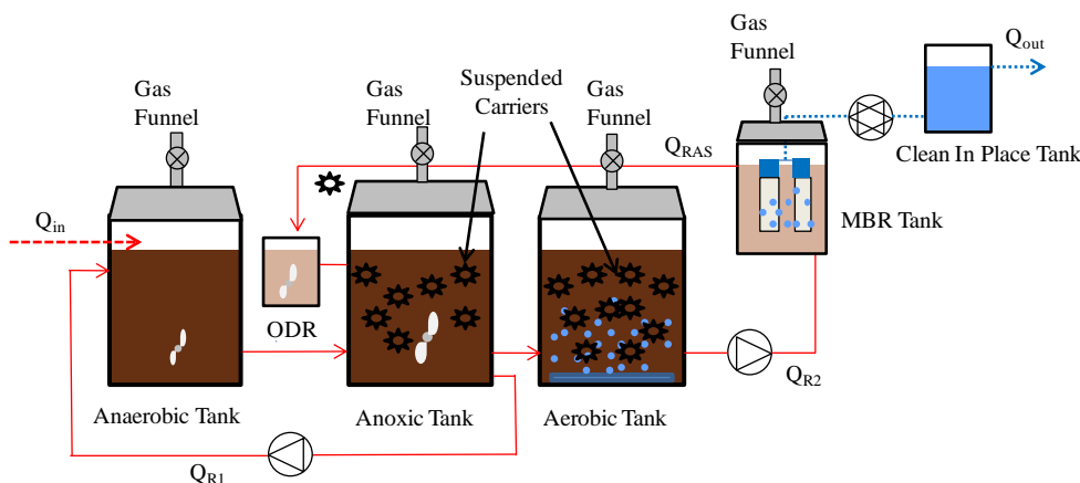
Figure 1. Schematic lay-out of the UCT-MBMBR pilot plant (Mannina et al., 2016b).
