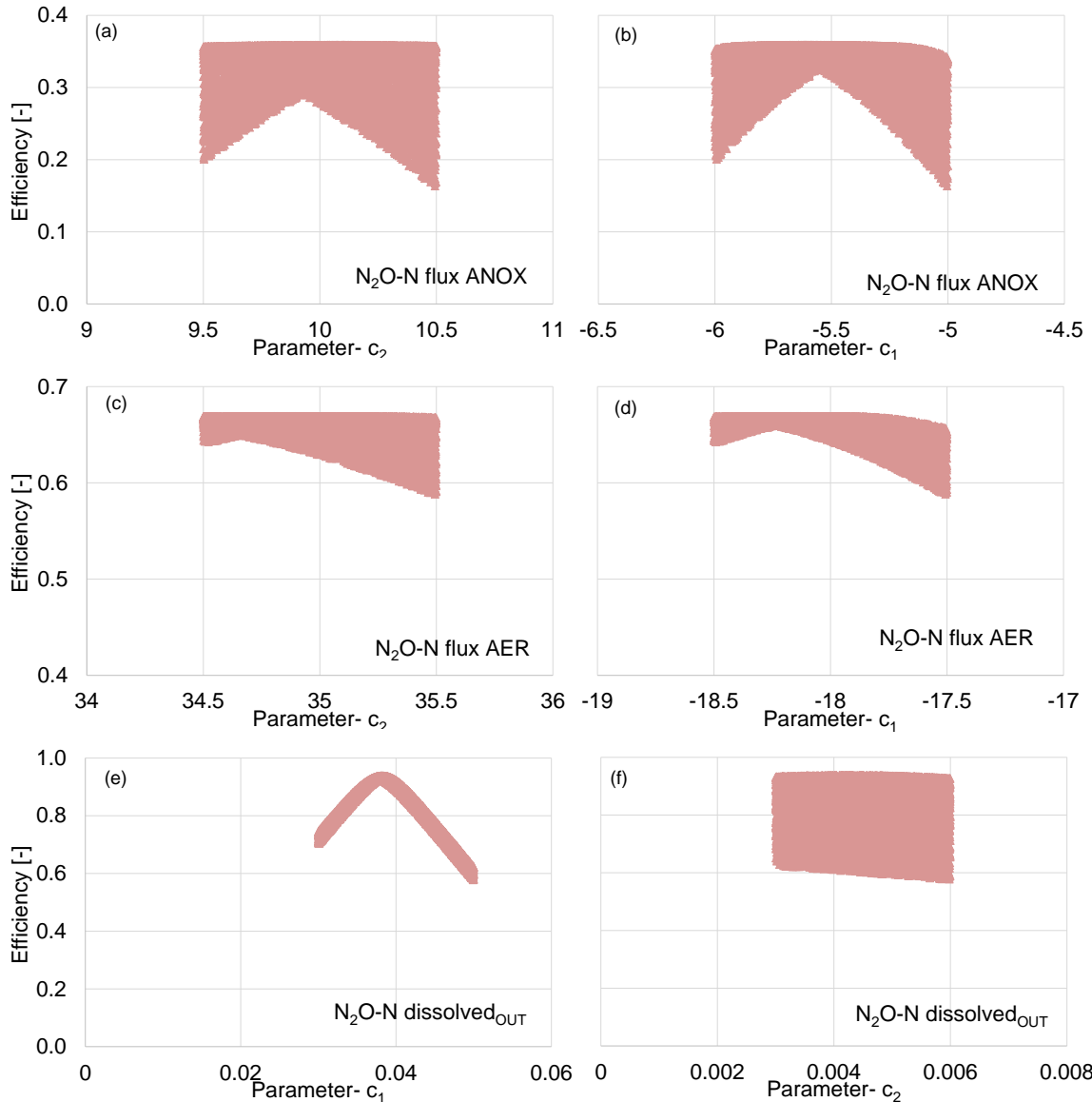
Figure 2. Scatterplot of N_2O-N flux ANOX (a, b), N_2O-N flux AER (c, d) and N_2O-N dissolved OUT (e, f) for the Phase III.
