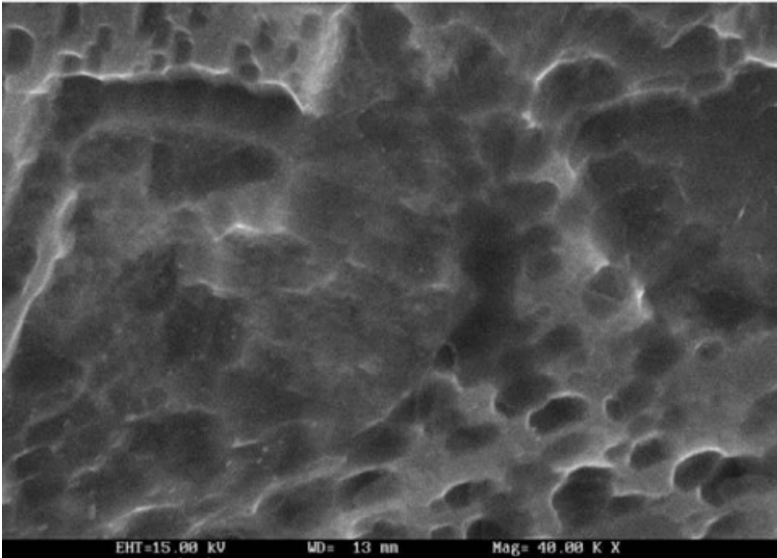
Figure 1. Image SEM (Scanning Electron Microscopy). Morphology of the surface of a porous stone sprayed with a 10% solution of lithium silicate which contains nanoparticles of silicon dioxide (~ 20 nm).
