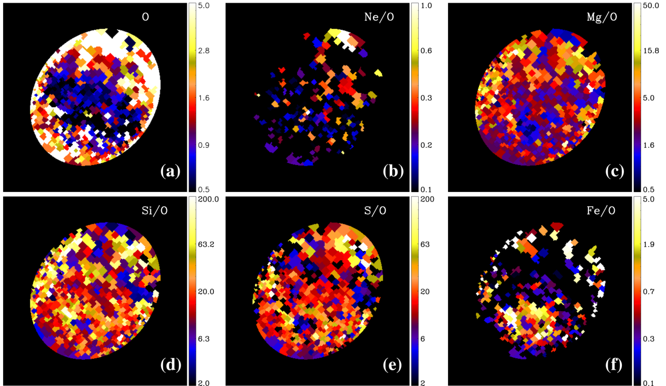
Figure 6. Abundance maps of the ejecta component. The oxygen abundance (a) is the absolute abundance in unit of solar, while the abundances of other elements are the abundance ratios to oxygen, also in unit of solar values.
