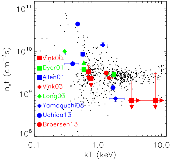
Figure 5. kT versus n_e t diagram. Black dots are the values of the ejecta component obtained from each region in the low-resolution run. Large coloured symbols are obtained from the literatures as denoted in the lower-left corner. For kT \gtrsim 2 keV, n_e t is in a narrow range, while for lower kT , n_e t is much more diverse.
