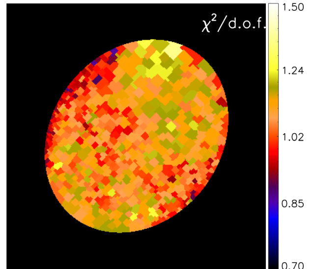
Figure 3. \chi^2/\text{d.o.f.} of the ‘2-T’ joint spectral fit of the low-resolution run. The maximum \chi^2/\text{d.o.f.} is 1.347, while the minimum value is 0.859.
