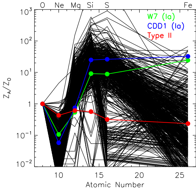
Figure 7. The relative abundances (to O) of different elements (Ne, Mg, Si, S, Fe) of the ejecta component. Data from the same region are connected together with a thin solid line. Theoretical model predictions of Type Ia (the classical deflagration model W7 and the delayed detonation model CDD1) and Type II (10–50 M_{\odot} ) SNe from Iwamoto et al. (1999) are plotted with large filled circles connected with thick solid lines. The O–Si abundances are in general consistent with the Type Ia SN products, but the observed Fe and sometimes S abundances are significantly lower than predicted by standard Type Ia SN yields.
