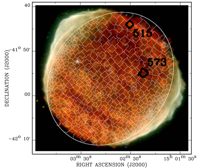
Figure 1. 583 tessellated meshes used for spatially resolved spectroscopy analysis overlaid on the tricolour images of SN1006 (red: 0.3–1 keV; green: 1–2 keV; blue: 2–8 keV). Each region contains \gtrsim 10^3 counts in 1.66–1.95 keV from the combination of MOS-1, MOS-2, and PN. The two regions marked in black are used to extract the example spectra shown in Fig. 2.
