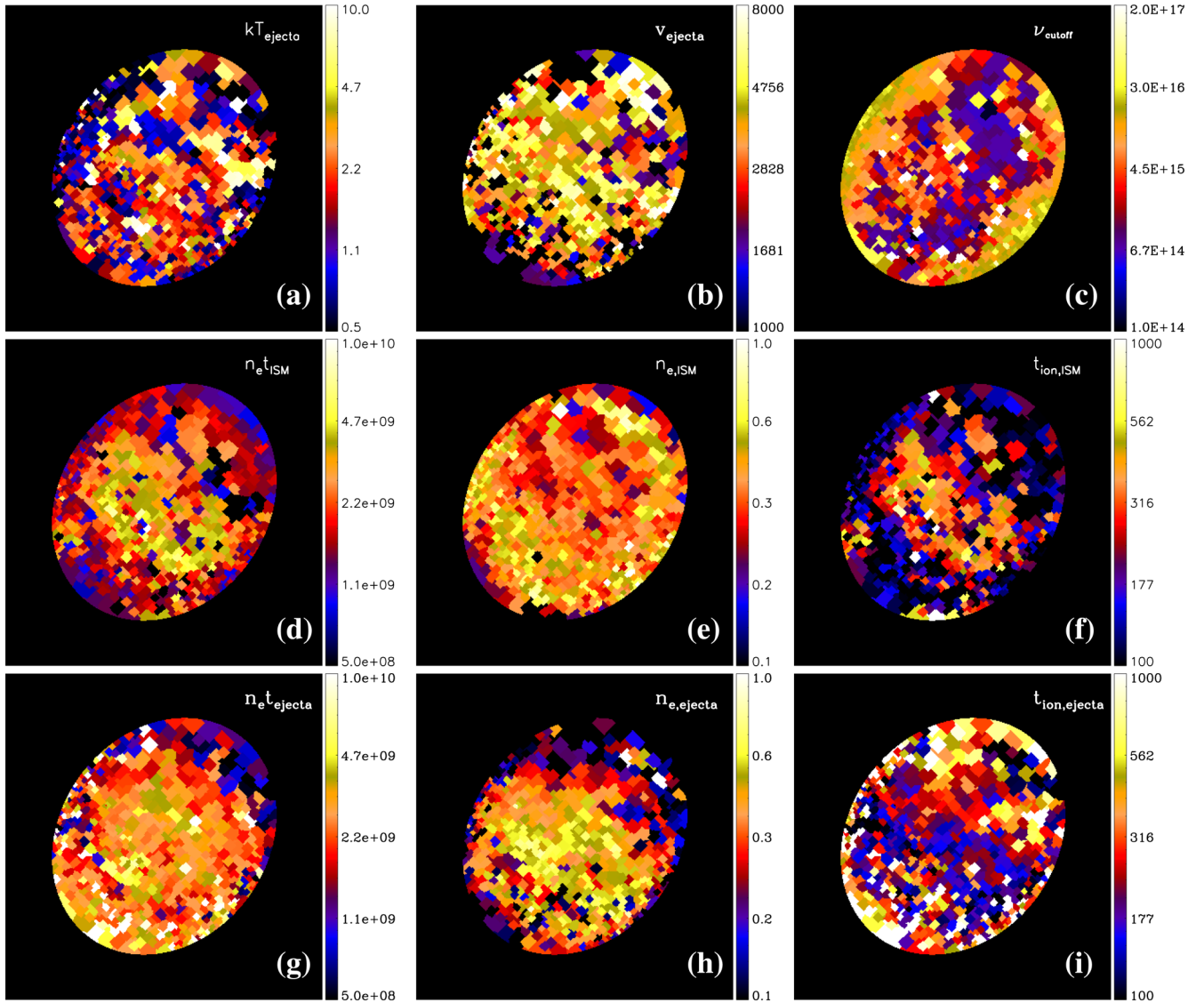
Figure 4. Parameter maps constructed by jointly analysing the spectra from the low-resolution meshes (Fig. 1) with the ‘2-T’ model. (a) Ejecta temperature in keV. (b) Line-of-sight velocity (positive towards the observer) in \text{km s}^{-1} . (c) Cutoff frequency of the non-thermal SRCUT component in Hz. (d–f) The ionization parameter in \text{cm}^{-3} \text{s} , electron number density in \text{cm}^{-3} , and ionization age in year of the ISM component. (g–i) Similar as (d–f), but for the ejecta component.
