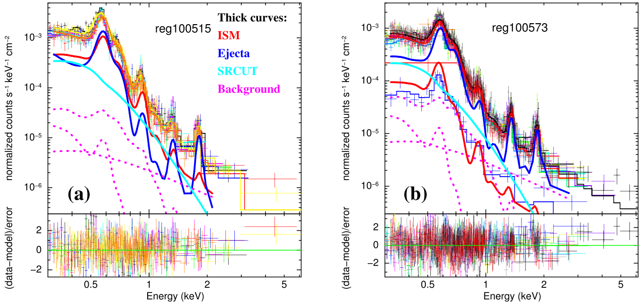
Figure 2. Example spectra extracted from the two regions marked in black in Fig. 1. Panel (a) shows an example with comparable contributions from the ISM and ejecta components, while panel (b) shows an example dominated by the ejecta emission. The coloured data points are the instrumental background-subtracted spectra extracted from different instruments (MOS-1, MOS-2, and PN) and different observations, while the thin solid curves with the corresponding colours are their best-fitting models (often not visible). Different model components are plotted as thick solid curves, as denoted on the top-right corner of panel (a). The Gaussian lines have too low flux to show up on both panels. The magenta dotted curves are the sky background components as detailed in the appendix of Paper I. The lower panels show the residuals of the fitting. The \chi^2/\text{d.o.f.} for the two panels are 1.168 (704.14/603) and 1.127 (1417.55/1258), respectively. Some of the best-fitting parameters and the corresponding errors are summarized in Table 1.
