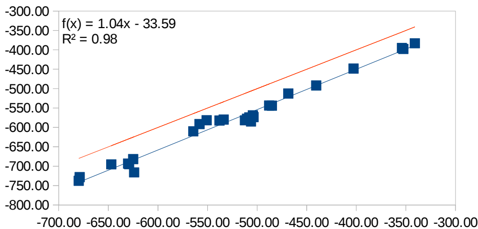
ADF: B3LY/TZ2P//OP2
