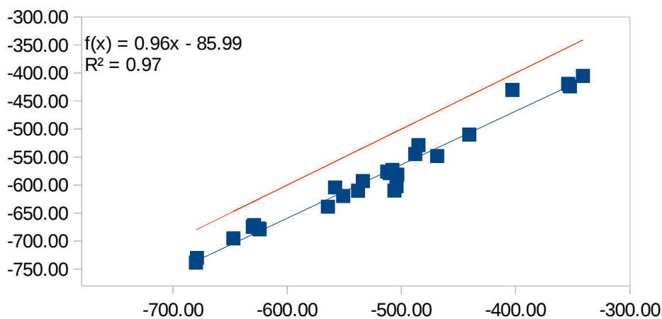
ADF SO-ZORA: B3LYP/DZP//OP3
