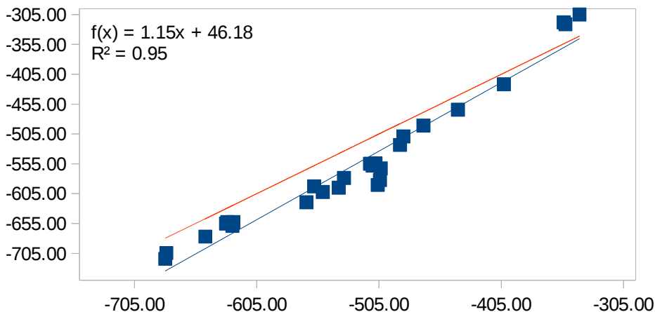
ADF Scalar ZORA: B3LYP/TZ2P//OP3
