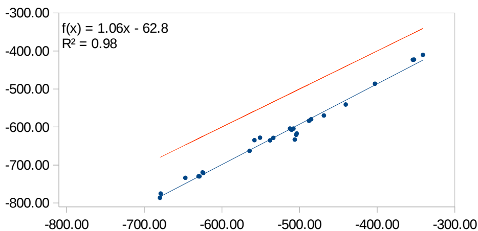
ADF SO-ZORA: B3LY/TZ2P//OP2
