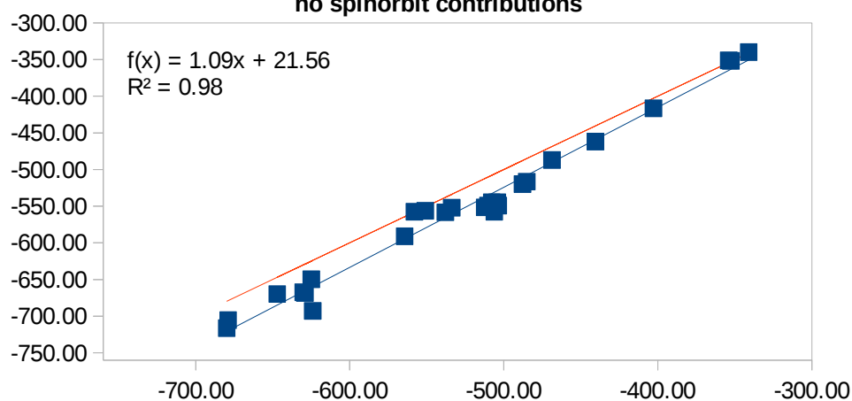
ADF SO-ZORA: B3LY/DZP/OP2 no spinorbit contributions
