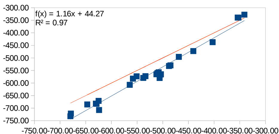
ADF Scalar-ZORA: B3LY/TZ2P//OP2
