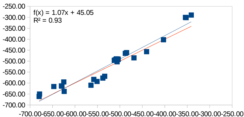
ADF Scalar ZORA: B3LYP/DZP//OP3
