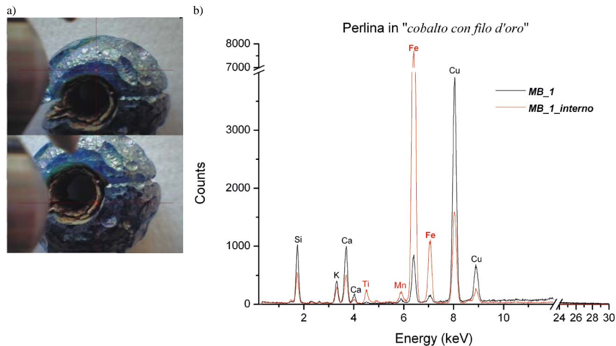
Fig 6. a) sample MB_1, cobalt bead b) XRF spectrum of the sample MB_1
