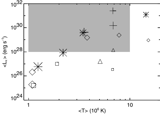
Fig. 10. Mean value of the X-ray luminosity as a function of the mean value of the best fit temperature, derived from our model synthesized spectra. Crosses correspond to Mach number M = 1000 , stars to M = 300 , diamonds to M = 100 , triangles to M = 30 and squares to M = 10 . The increasing size of each symbol corresponds to increasing value of the ambient medium-to-jet density contrast, \nu = 0.01-300 . The shaded region refers to the (L_X, T) values consistent with observations of HH objects in general.
