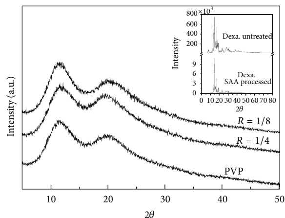
FIGURE 7: XRPD related to the PVP untreated and PVP microparticles produced by SAA using different solvents.
