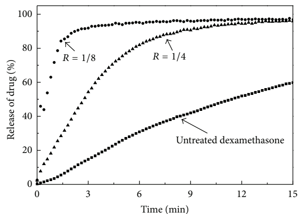
FIGURE 6: Dissolution rate of dexamethasone-PVP composite particles produced by SAA with respect to the untreated drug, in physiological solution.
