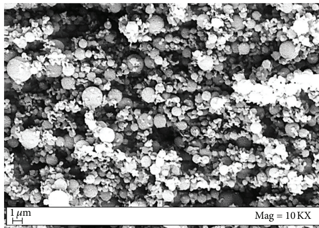
FIGURE 3: Dexamethasone microparticles obtained by SAA at 40°C and 76 bar in the saturator and 70°C and 1.6 bar in the precipitator.
