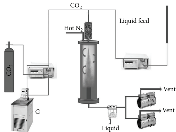
FIGURE 1: Scheme of SAA plant. G is the cool bath to cold the head of high pressure pump.
