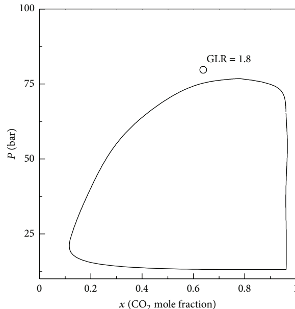
FIGURE 2: Vapor liquid equilibria for the system ethanol-CO 2 at 40°C. Adapted from Knez et al. [22].
