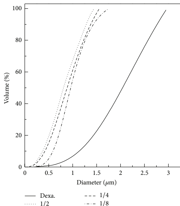
FIGURE 5: Volumetric cumulative particle size distribution of dexamethasone-PVP composite particles produced by SAA at different drug/polymer ratios.
