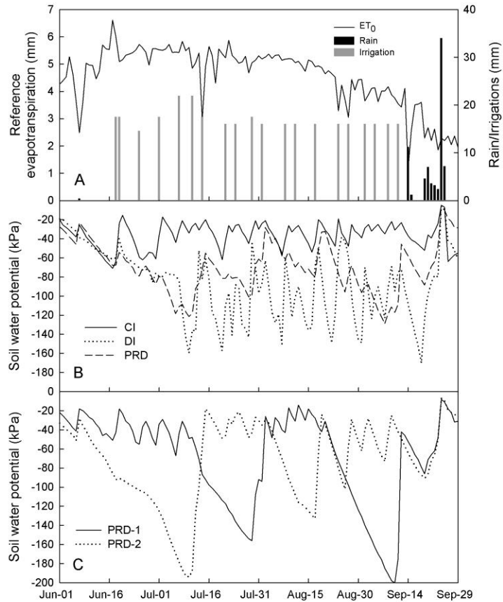
Fig. 2.3. Water losses and inputs (A) recorded in summer 2008 at the experimental site in Palermo (30°06' N, 13°21' E, and 31 m a.s.l.), Sicily. Soil water potential in the rootzone of 'Valencia' orange trees under conventional irrigation (CI), continuous deficit irrigation (DI), and partial rootzone drying (PRD, average of wet and dry side; panel B) and in the two sides of the rootzone of trees under PRD (C) during the 2008 irrigation season.
