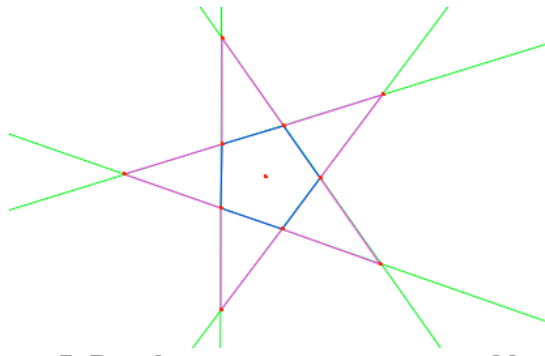
Figure 7: Regular star pentagon generated by extending sides of another polygon
