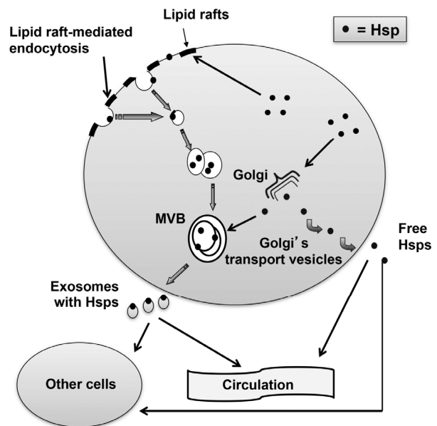
Figure 1. Pathways of secretion of heat shock proteins (Hsps) by tumour cells. Cytosolic Hsps can be released in free, soluble forms by Golgi transport vesicles or can be bound to exosomes. The latter is produced by multivesicular bodies (MVB) fusing with the plasma membrane of cells. Lipid rafts participate in Hsps release by exosomes, as they are internalized by endocytosis, which for various reasons reach the plasma membrane of tumour cells, and enter into MVB. Secreted Hsps may interact with other cells in the peritumoural environment or be released into the bloodstream.
